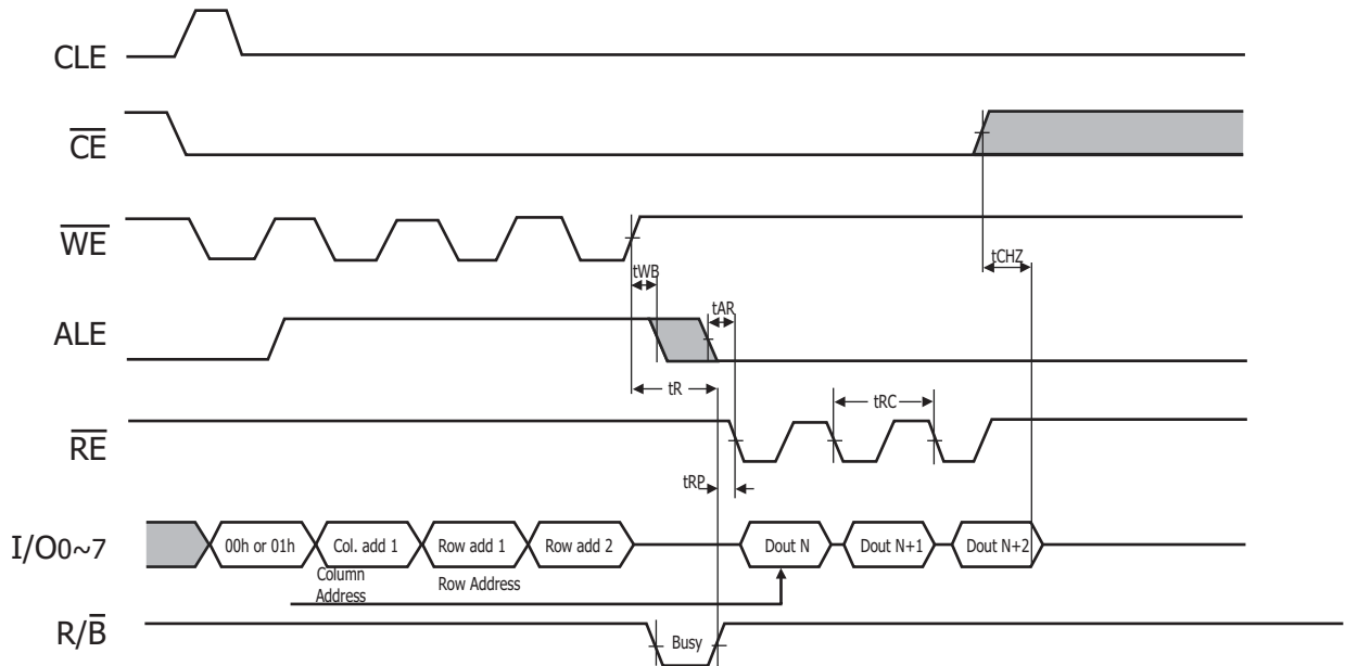
Figure 11: Read1 Operation intercepted by CE#
