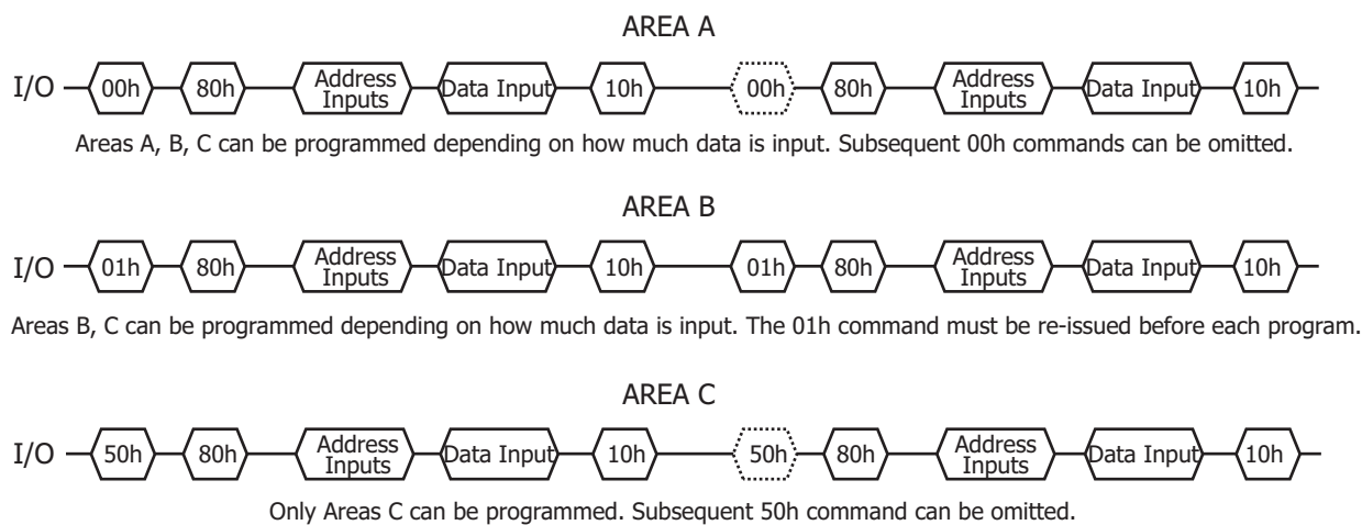
Figure 28: Pointer Operations for porgramming
