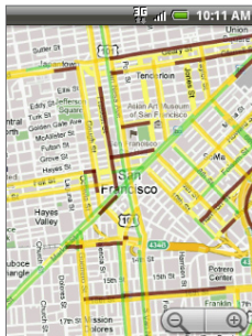
Traffic mode
