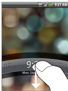
Lock screen
