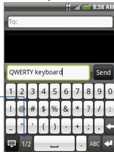
QWERTY keyboard
