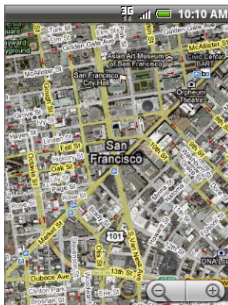
Satellite mode
