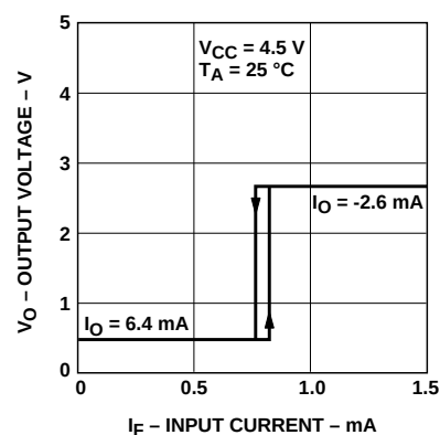
Figure 3. Typical Output Voltage vs. Forward Input Current.
