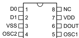
HT6P20B – 8 DIP/SOP
