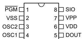
HT6P20A – 8 DIP/SOP
