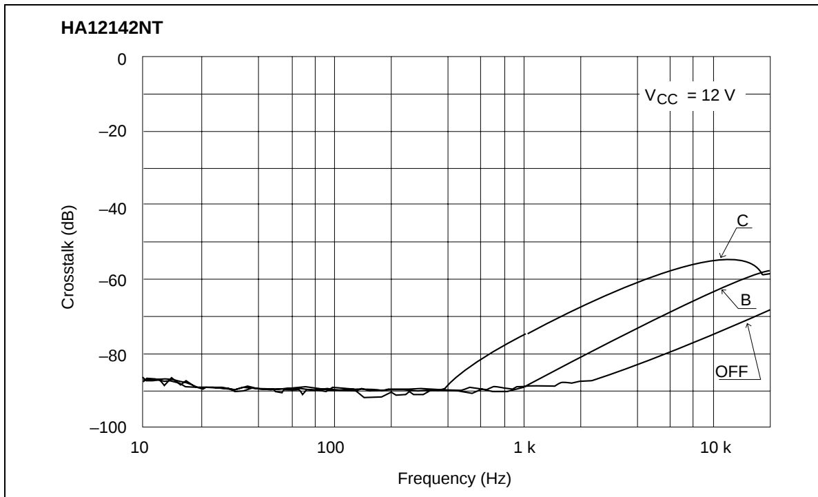
Crosstalk vs. Frequency (PB→REC)
