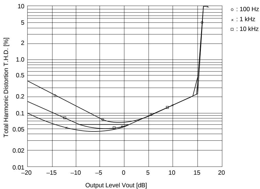
Total Harmonic Distortion vs. Output Level (PB MODE NR-B V_{CC} = 14 V)
