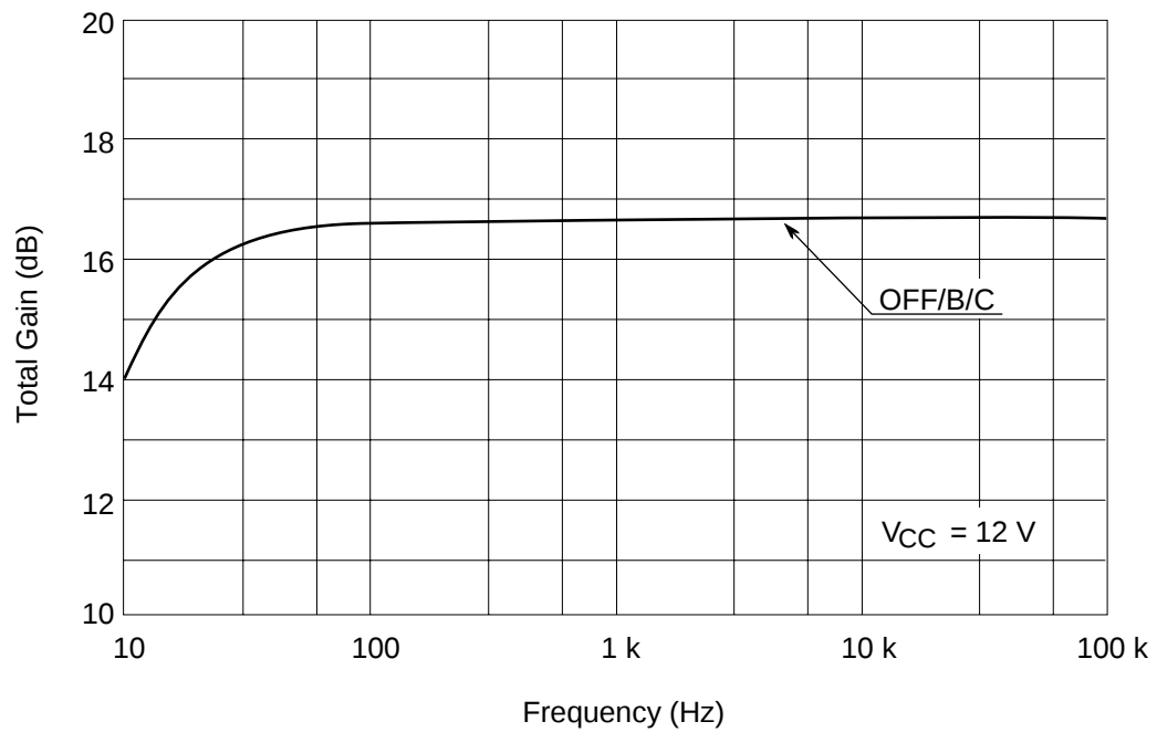
Total Gain vs. Frequency (REC MODE PBOU)
