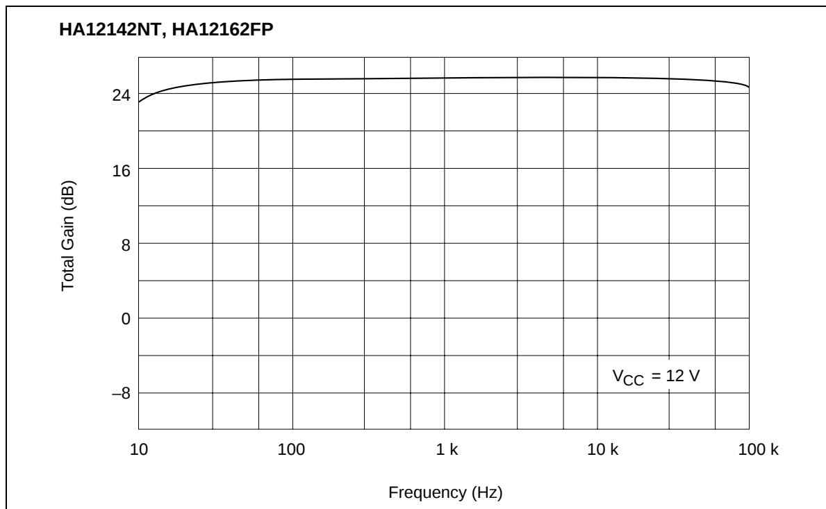
Total Gain vs. Frequency (PB MODE PBOU NR-OFF)
