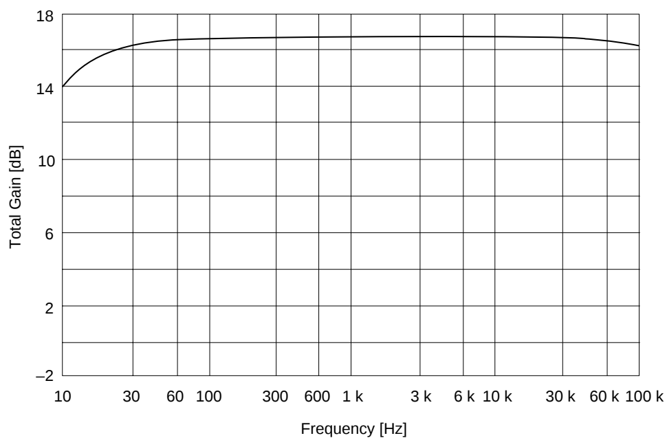
Total Gain vs. Frequency (REC MODE RECOUT NR-OFF V_{CC} = 14\text{ V} )
