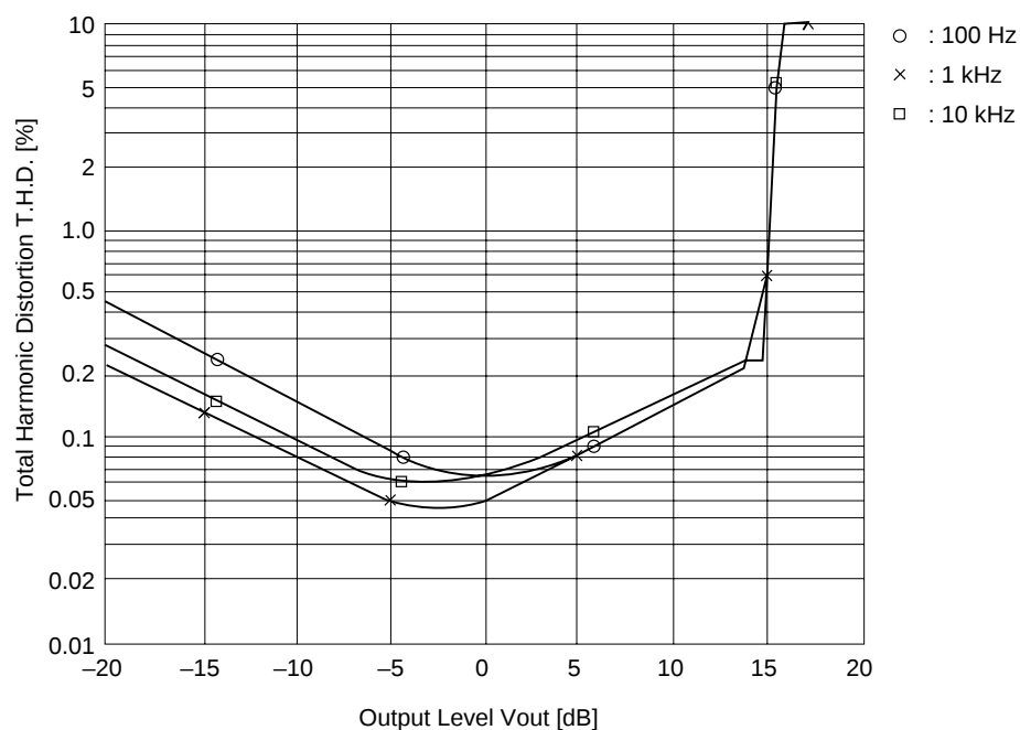
Total Harmonic Distortion vs. Output Level (PB MODE NR-OFF V_{CC} = 14 V)
