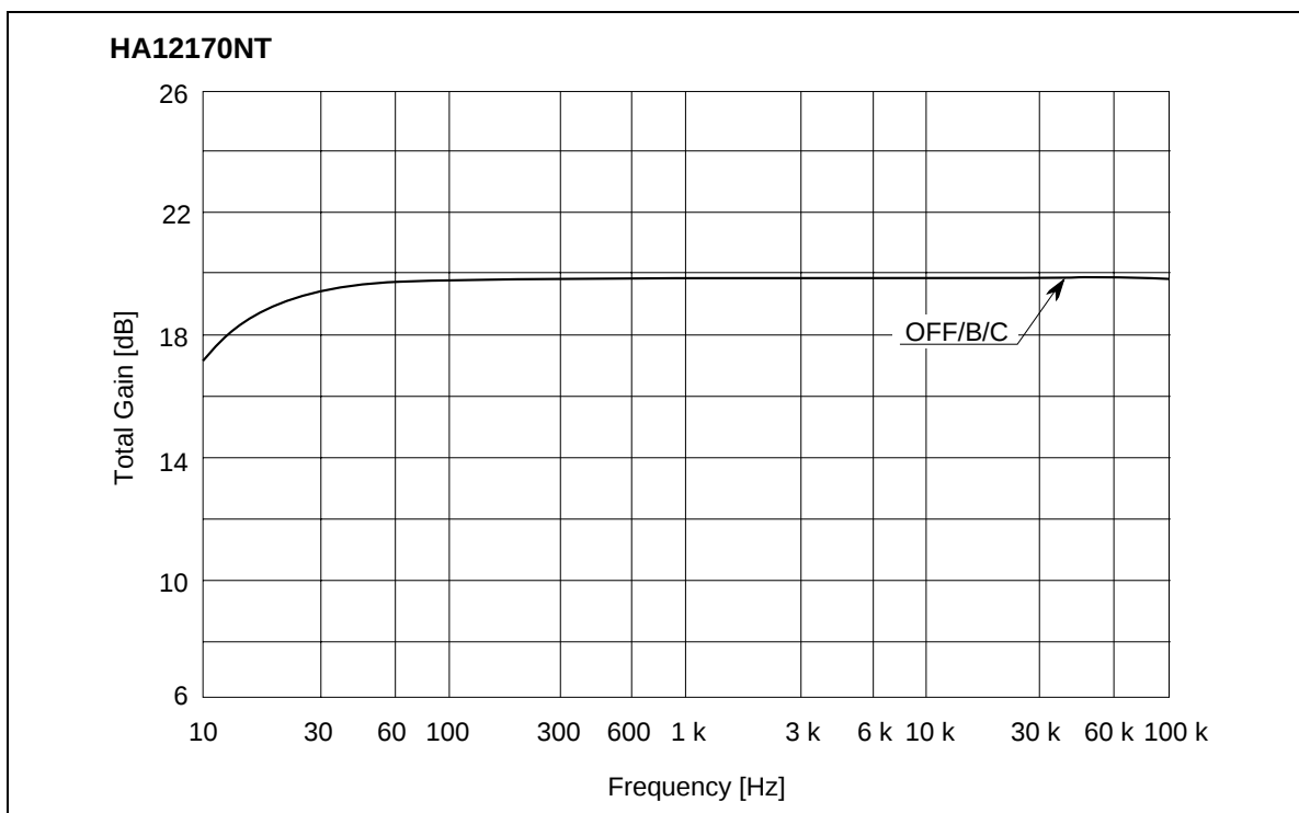
Total Gain vs. Frequency (PB MODE RECOUNT V_{cc} = 14 V)
