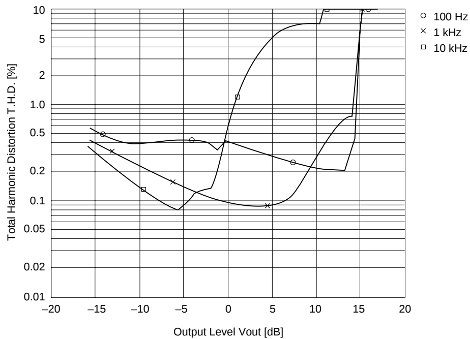
Total Harmonic Distortion vs. Output Level (REC MODE NR-C V_{cc} = 14 V)
