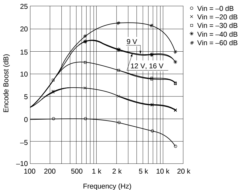
Encode Boost vs. Frequency (NR-C, V_{cc} = 9 \text{ V}, 12 \text{ V}, 16 \text{ V} )
