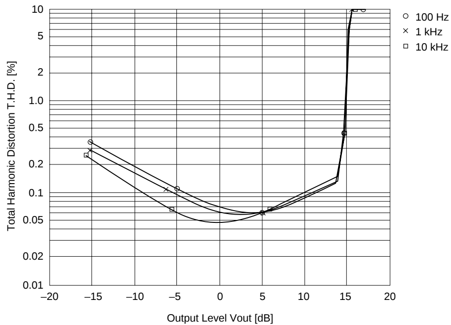
Total Harmonic Distortion vs. Output Level (REC MODE NR-B V_{cc} = 14 V)
