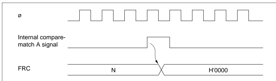
Figure 8.7 Clearing of FRC by Compare-Match A
