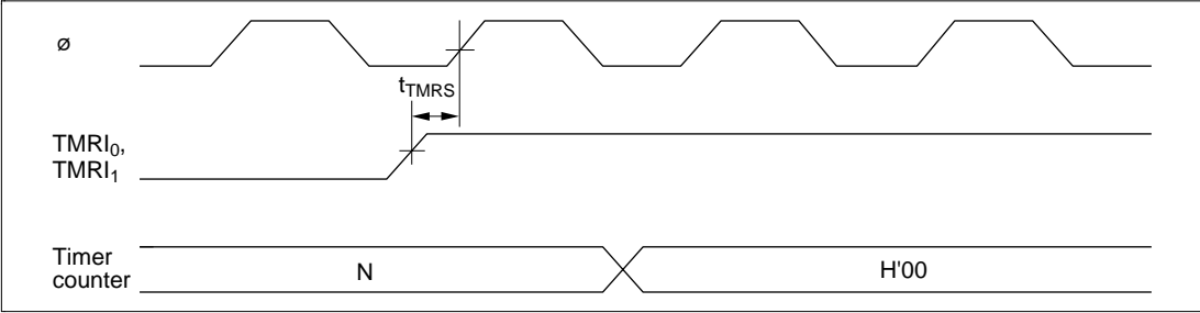
Figure 23.17 8-Bit Timer Reset Input Timing
