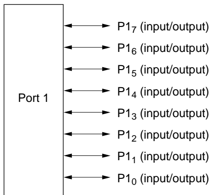
Figure 7.4 Pin Functions in Mode 3 (Port 1)
