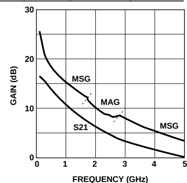
Figure 20. AT-32033 Gains vs. Frequency at V_{CE} = 2.7\text{ V}, I_C = 2\text{ mA} .
