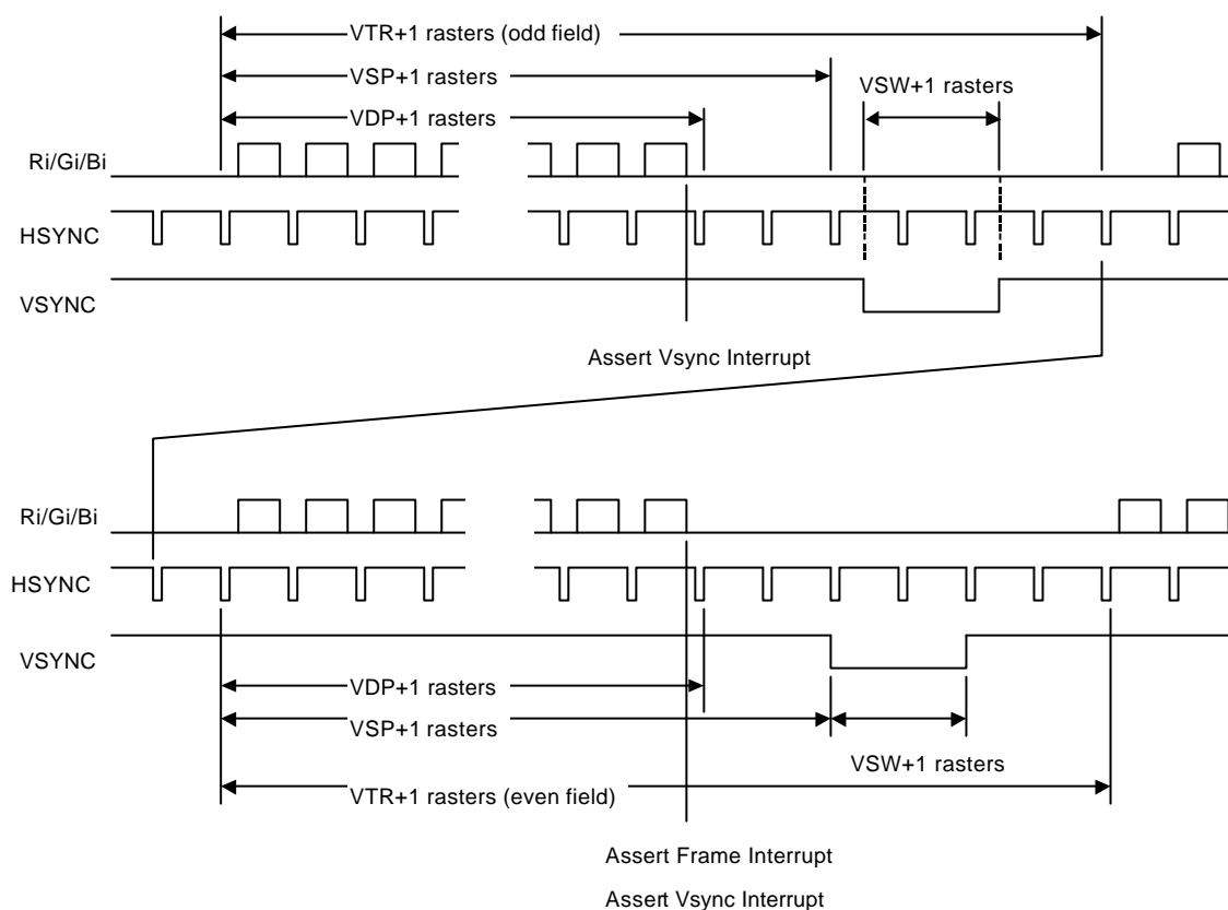
Fig. 10.27 Interlace Video Timing
