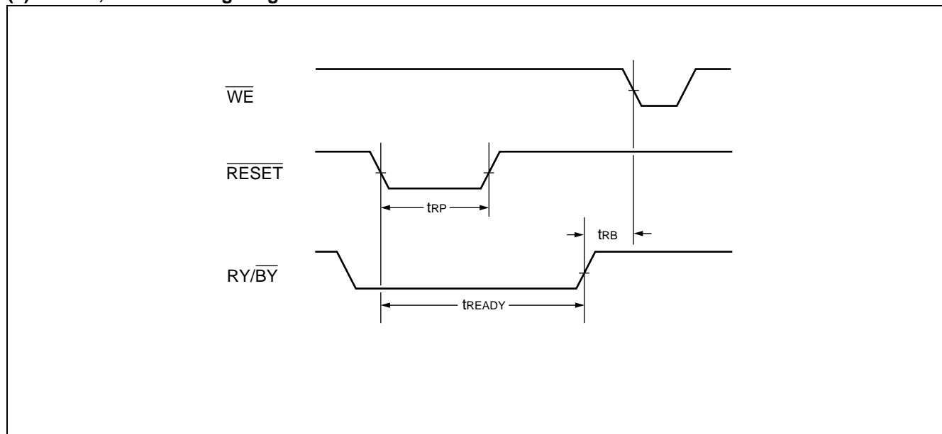
(9) RESET, RY/ \overline{\text{BY}} Timing Diagram
