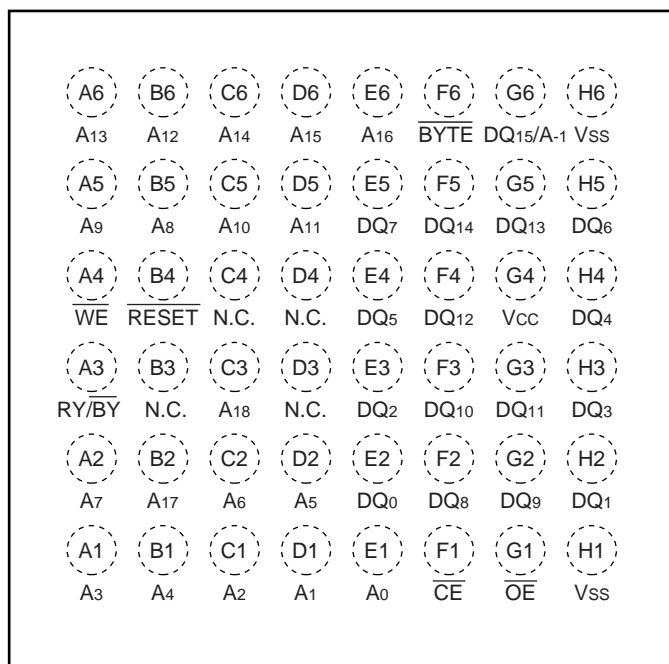
FBGA (TOP VIEW) Marking side
