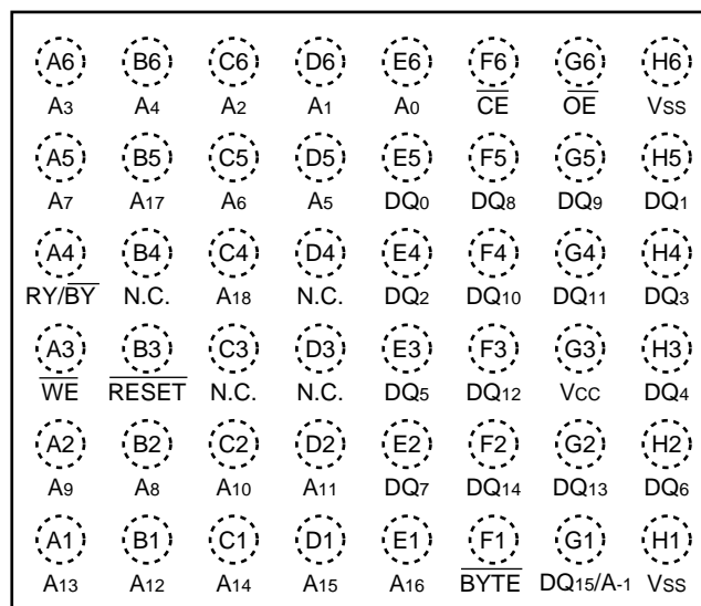
SCSP (TOP VIEW) Marking side
