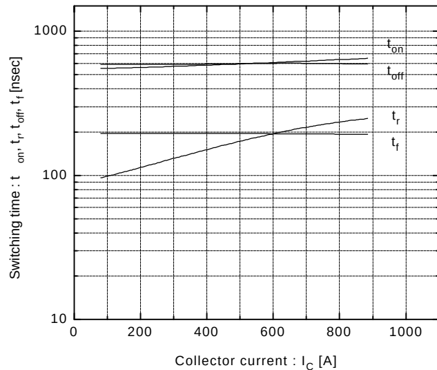
Switching time vs. Collector current V_{CC}=300\text{V} , R_G=2.7\Omega , V_{GE}=\pm 15\text{V} , T_J=25^\circ\text{C}
