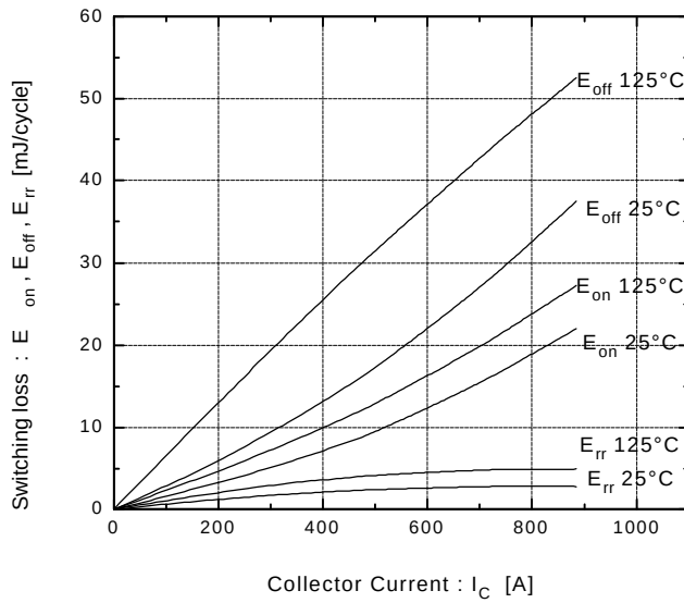
Switching loss vs. Collector current
