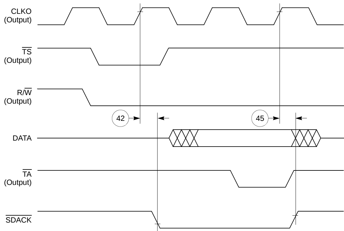
Figure 44. SDACK Timing Diagram—Peripheral Read, Internally-Generated TA
