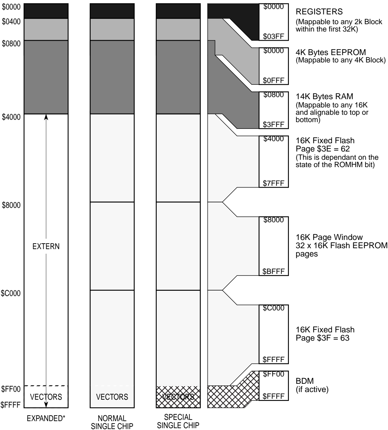
Figure 1-2 MC9S12DP512 Memory Map
