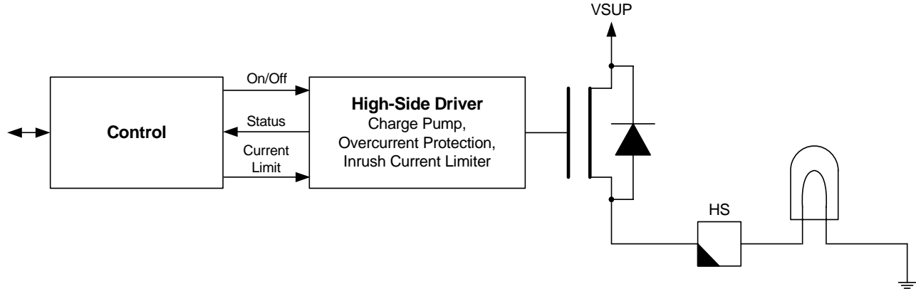
Figure 21. High-Side Circuitry
