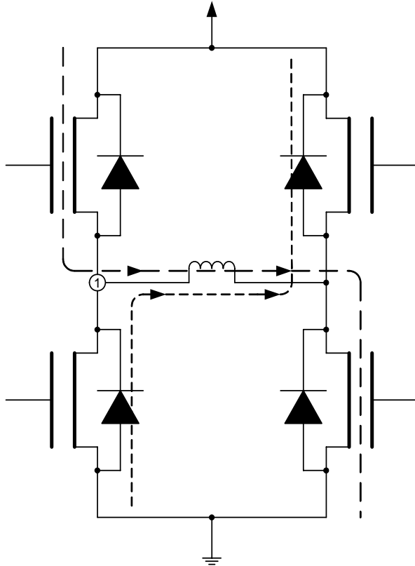
Figure 20. BEMF Signal Generation
