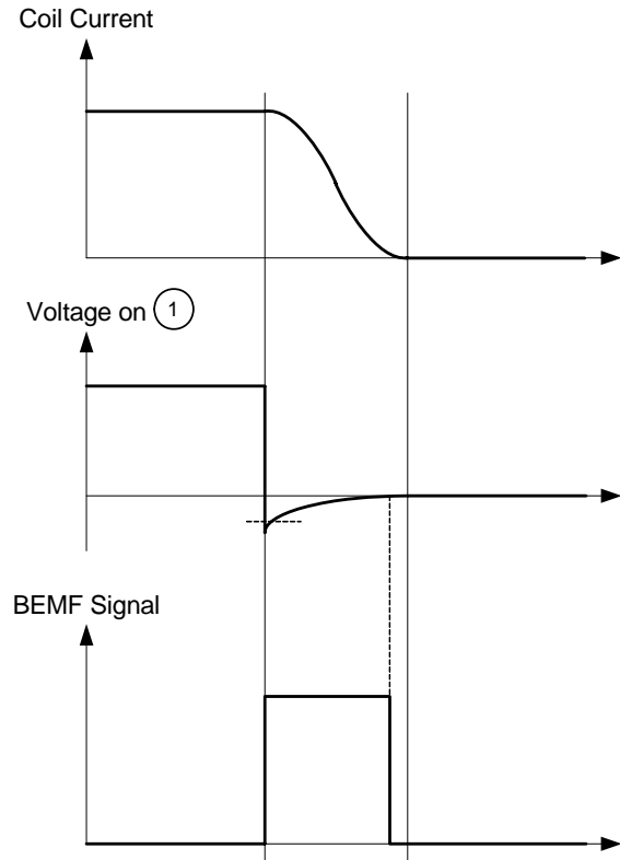
Figure 20. BEMF Signal Generation
