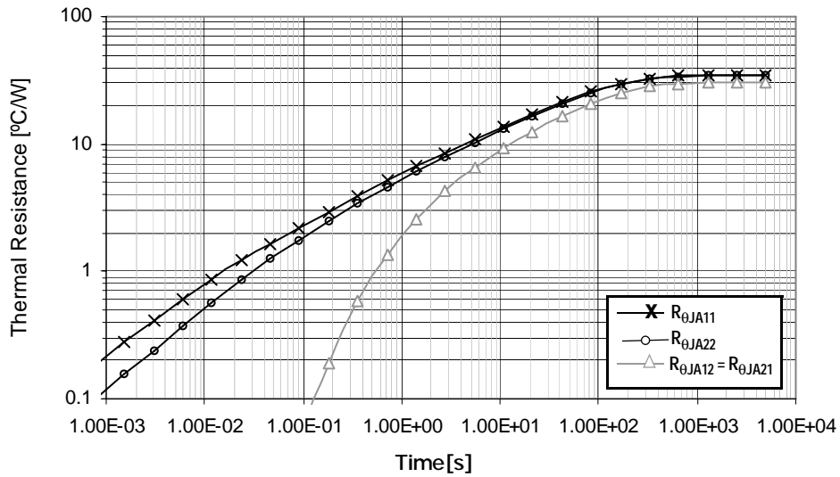
Figure 30. Transient Thermal Resistance R_{\theta JA} (1.0 W Step Response) Device on Thermal Test Board Area A = 600 (mm²)
