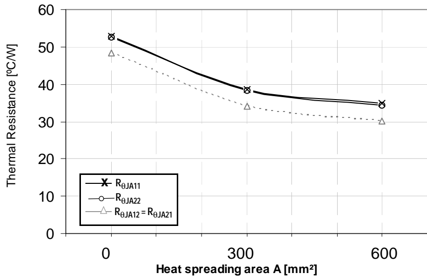
Figure 29. Device on Thermal Test Board R_{\theta JA}
