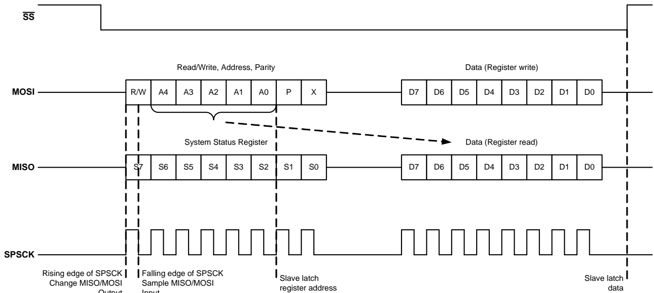
Figure 9. SPI Protocol
