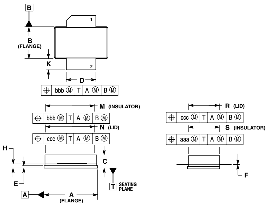
CASE 465C-02 ISSUE A NI-880S MRF5S19150HSR3
