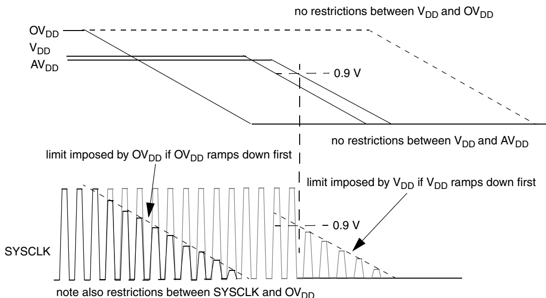
Figure 17. MPC7448 Power Down Sequencing Requirements
