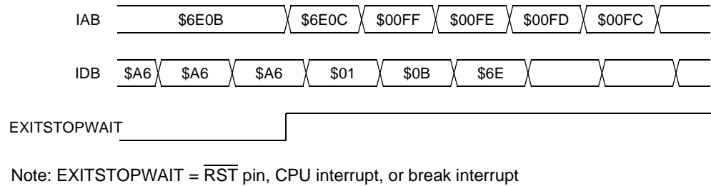
Figure 19-16. Wait Recovery from Interrupt or Break
