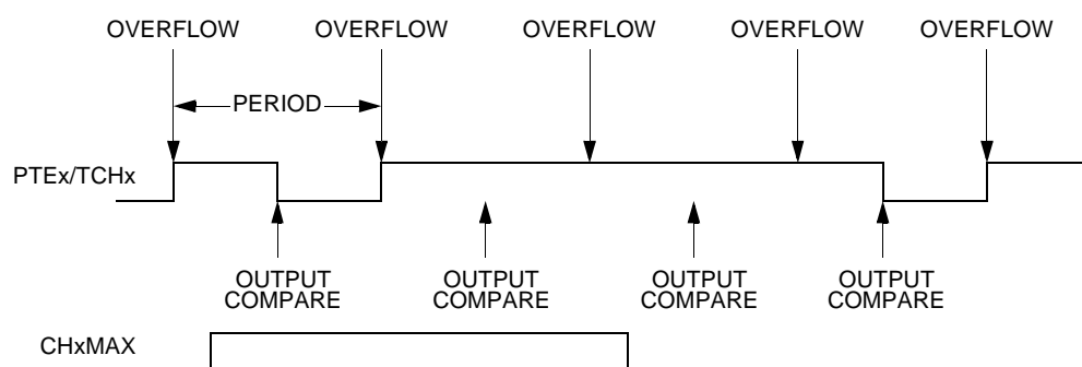
Figure 22-13. CHxMAX Latency
