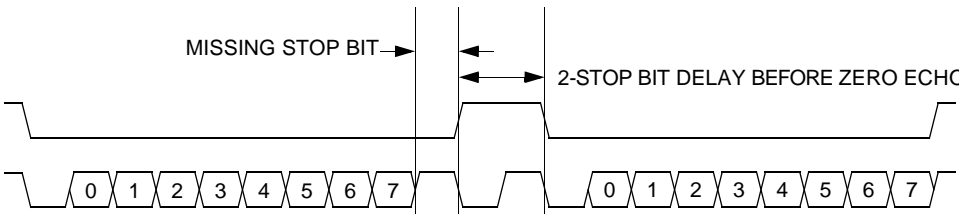
Figure 15-4. Break Transaction
