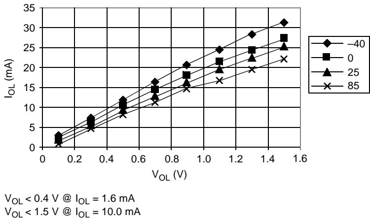
Figure 23-11. Typical Low-Side Driver Characteristics – Ports PTB5–PTB0, PTD6–PTD0, and PTE1–PTE0 ( V_{DD} = 5.5 \text{ Vdc} )
