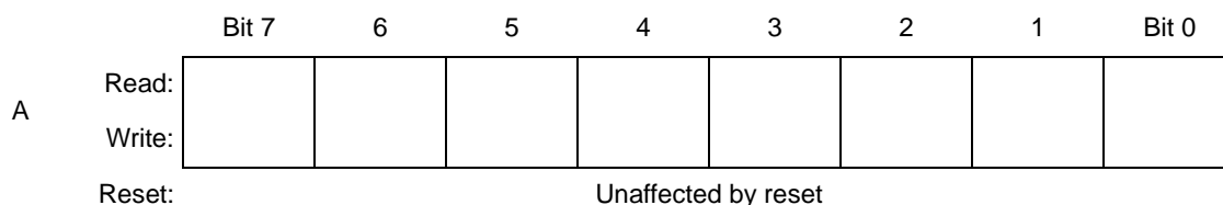
Figure 10-2. Accumulator (A)
