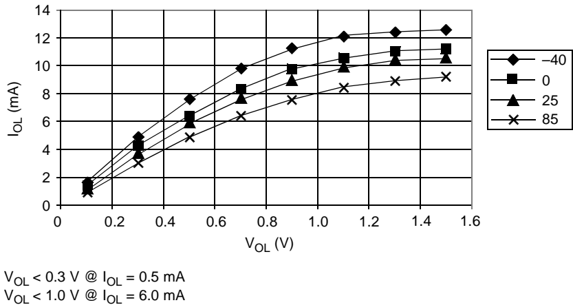
Figure 23-12. Typical Low-Side Driver Characteristics – Ports PTB5–PTB0, PTD6–PTD0, and PTE1–PTE0 ( V_{DD} = 2.7 \text{ Vdc} )
