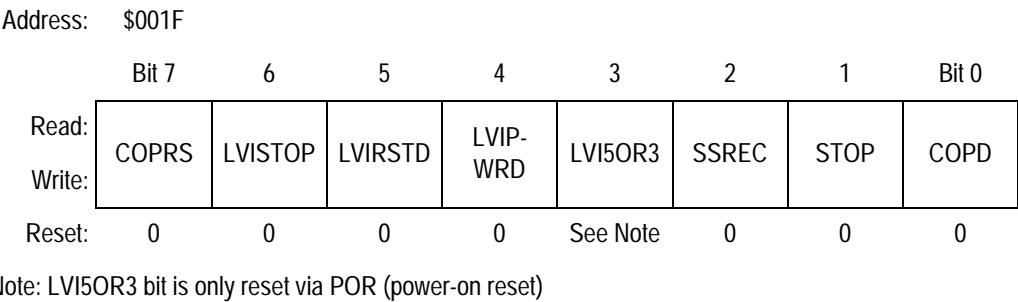
Figure 8-2. Configuration Register 1 (CONFIG1)
