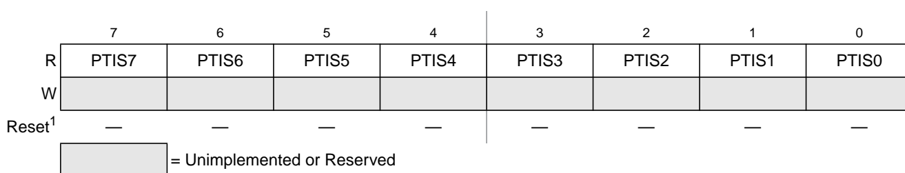
Figure 24-22. Port S Input Register (PTIS)
