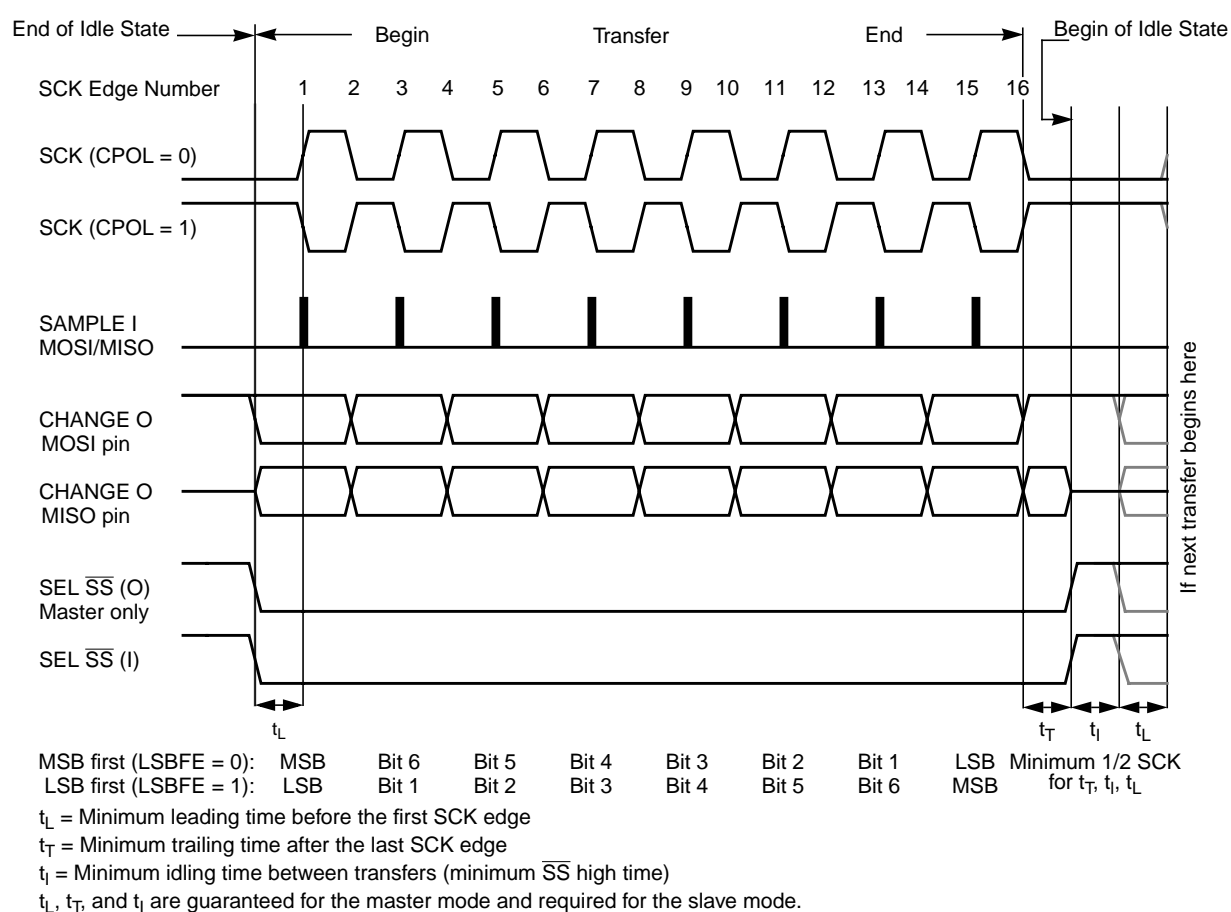
Figure 12-11. SPI Clock Format 0 (CPHA = 0)
