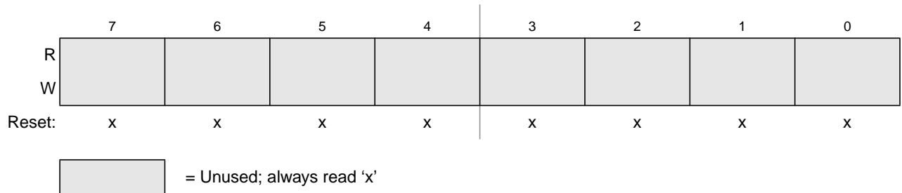
Figure 10-32. Identifier Register 2 — Standard Mapping
