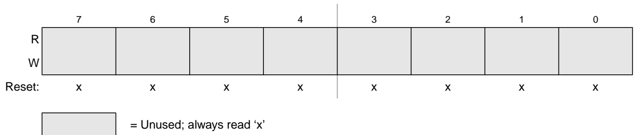
Figure 10-33. Identifier Register 3 — Standard Mapping
