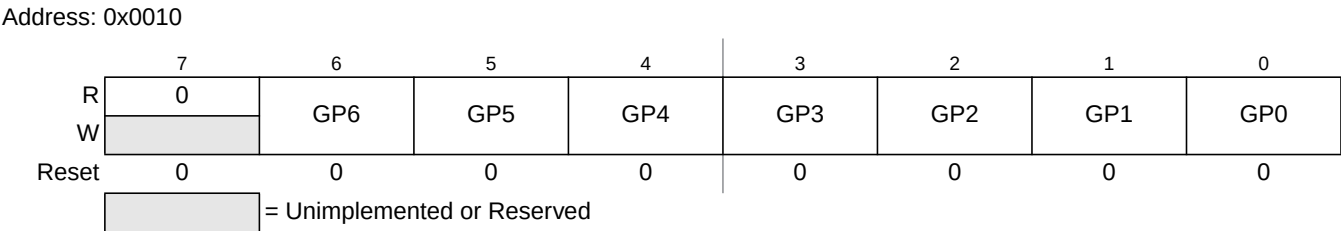
Figure 18-6. Global Page Index Register (GPAGE)
