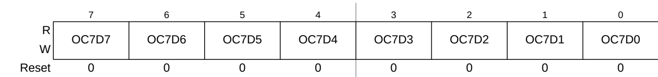
Figure 7-6. Output Compare 7 Data Register (OC7D)
