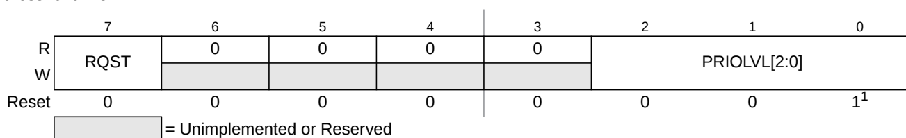
Figure 16-6. Interrupt Request Configuration Data Register 0 (INT_CFDATA0)
