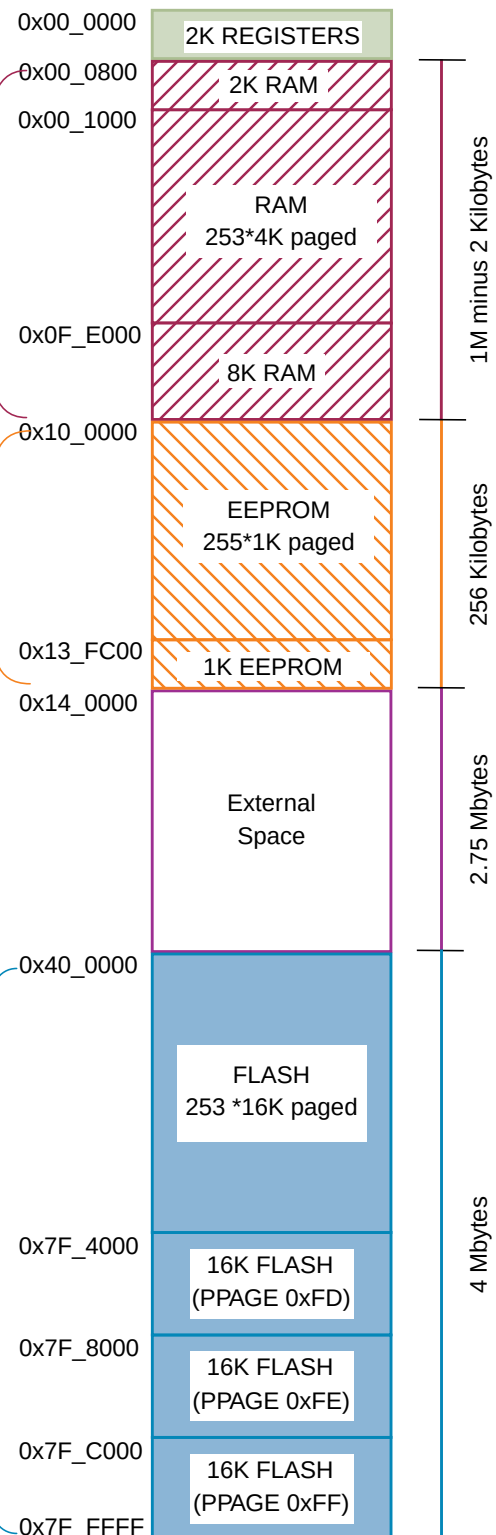
Figure 18-21. Expansion of the Local Address Map
