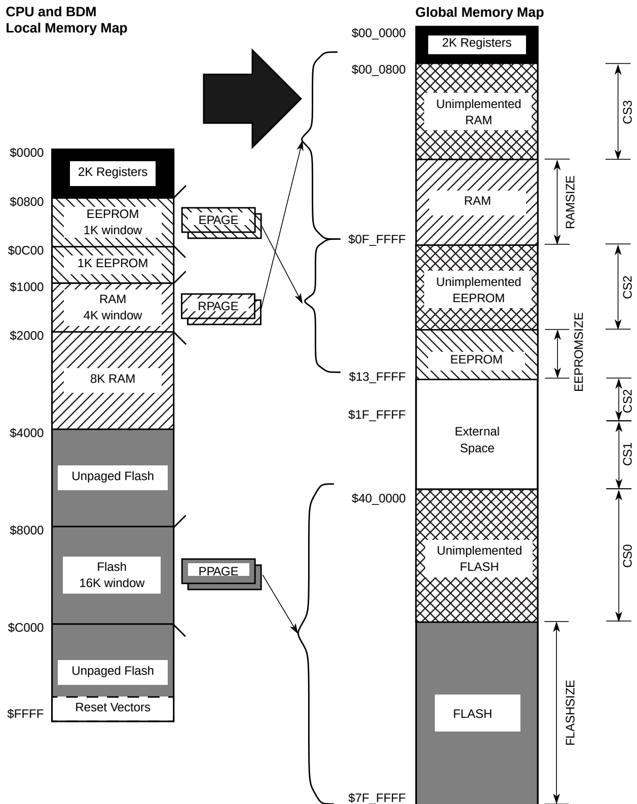
Figure 17-23. Local to Implemented Global Address Mapping (Without GPAGE)
