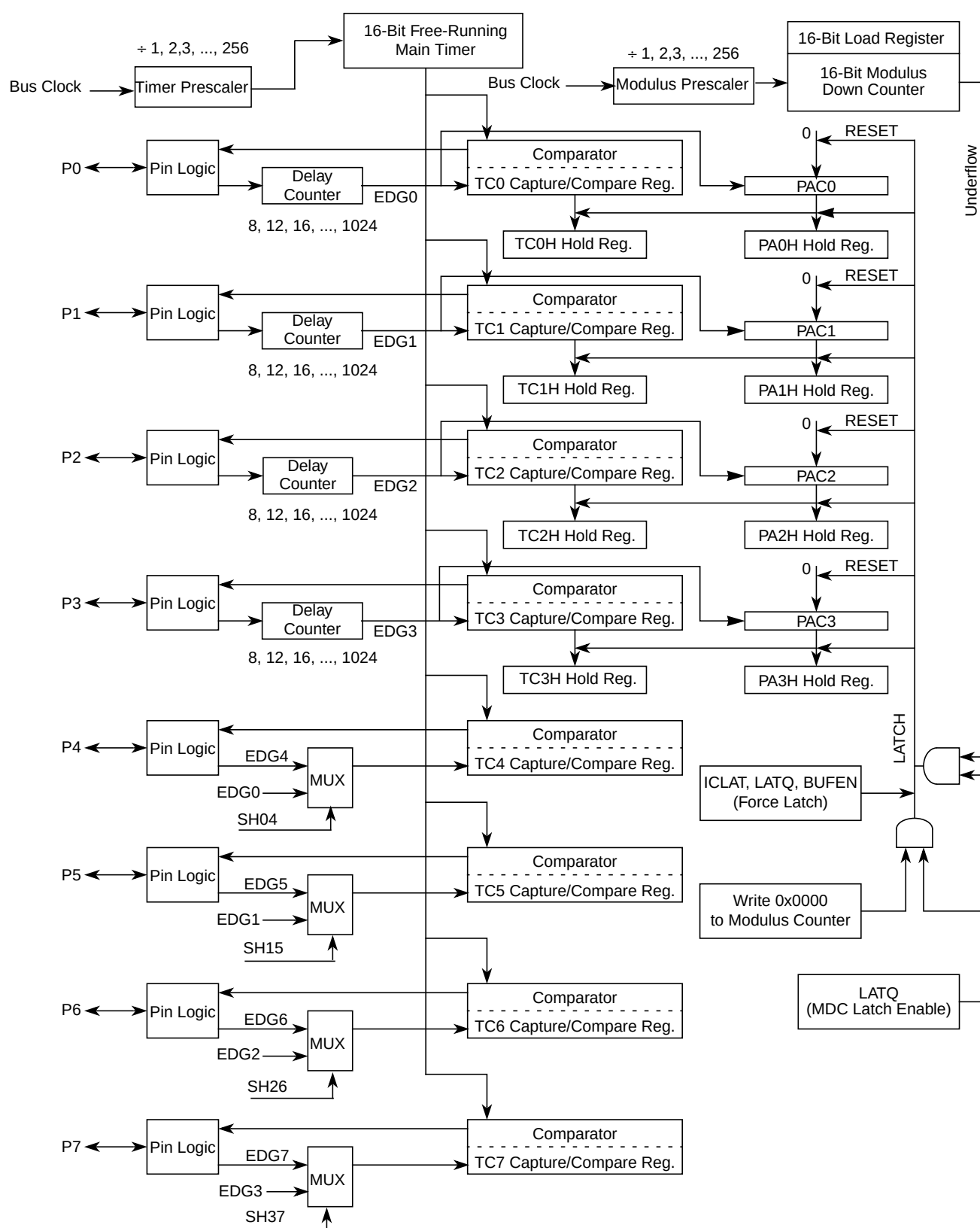
Figure 7-66. Detailed Timer Block Diagram in Latch Mode when PRNT = 1
