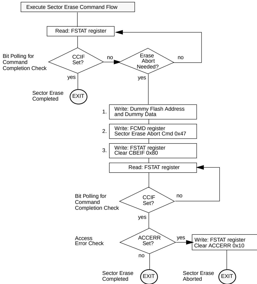
Figure 29-29. Example Sector Erase Abort Command Flow
