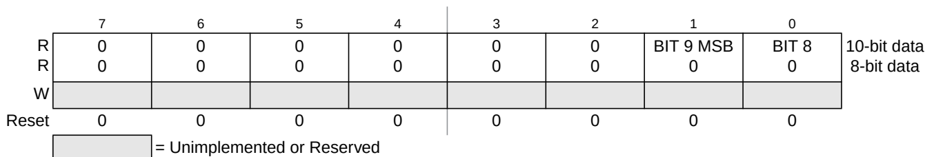
Figure 5-17. Right Justified, ATD Conversion Result Register, High Byte (ATDDR x H)
