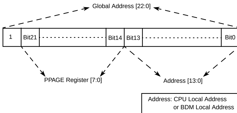
Figure 18-16. PPAGE Address Mapping
