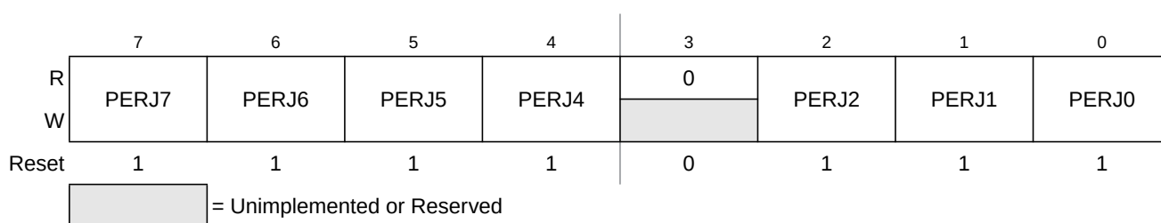
Figure 23-60. Port J Pull Device Enable Register (PERJ)
