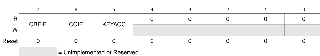
Figure 29-7. Flash Configuration Register (FCNFG)
