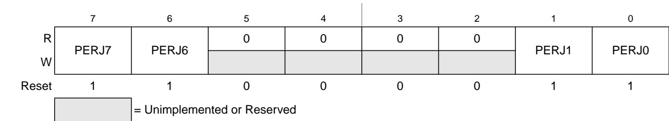
Figure 24-56. Port J Pull Device Enable Register (PERJ)
