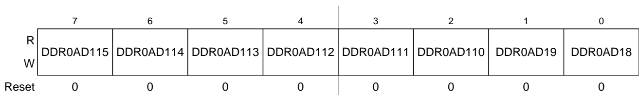
Figure 24-62. Port AD1 Data Direction Register 0 (DDR0AD1)
