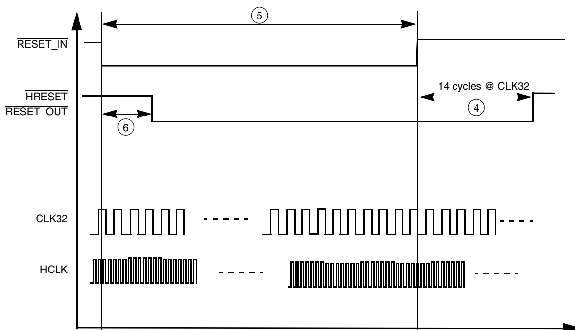
Figure 4. Timing Relationship with RESET_IN
