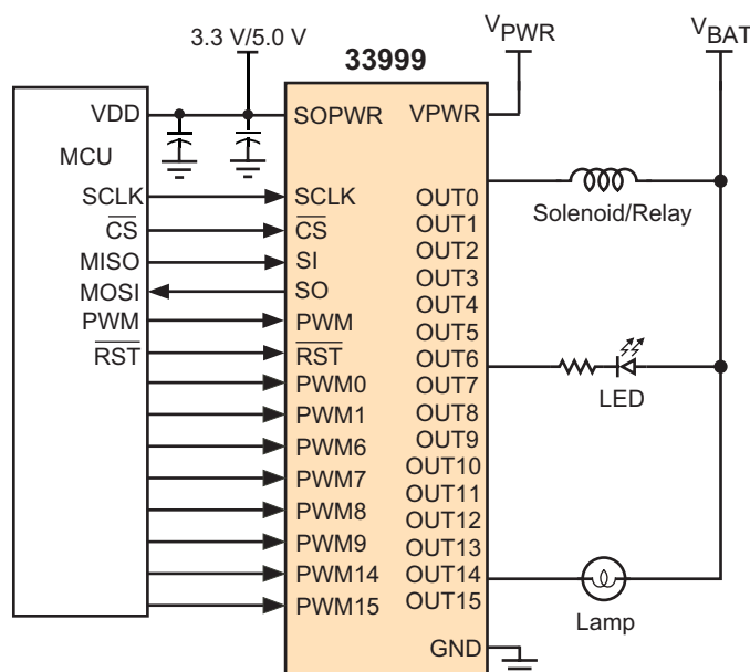
Figure 1. 33999 Simplified Application Diagram
