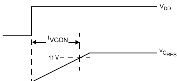
Figure 7. Charge Pump Timing
