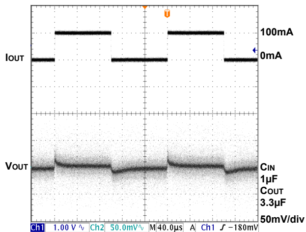
LOAD TRANSIENT
