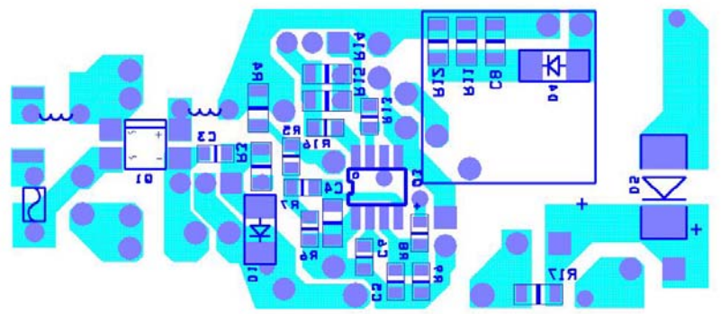
Figure 9. Printed PCB, Bottom Side
