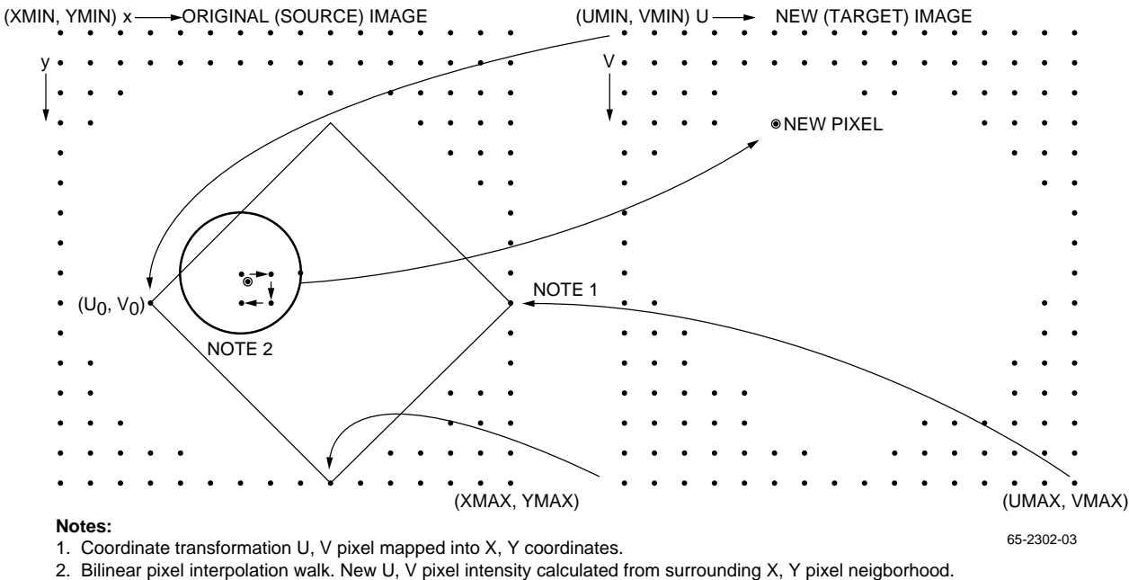
Figure 1. Image resampling geometry showing two-dimensional image rotation and expansion
