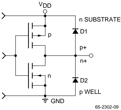
Figure 6. Equivalent Output Circuit
