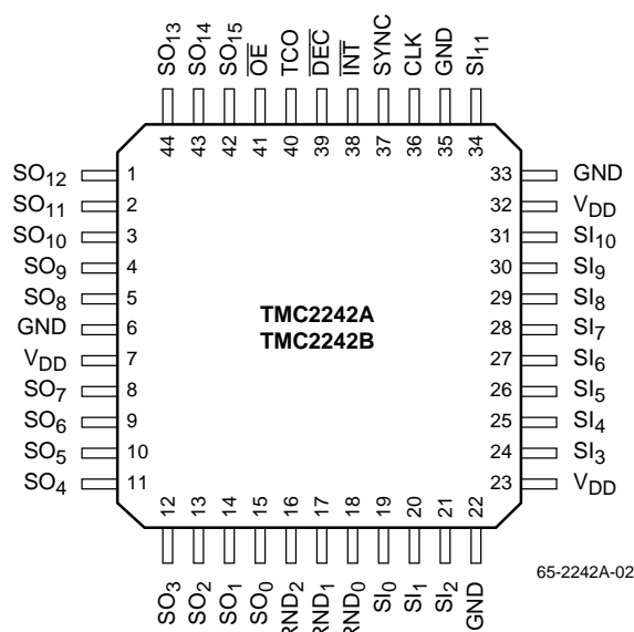
44 Lead MQFP
