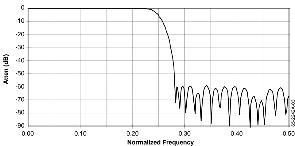
Figure 1. Frequency Response
