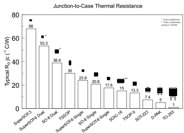
Figure 8. Junction-to-case thermal resistance R_{\theta JC} of various surface mount Power MOSFET packages.
