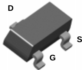
Figure 1. SuperSOT™-3 Power MOSFET has the same package dimensions as the SOT-23 but the maximized copper lead frame reduces the junction-to-case thermal resistance R_{\theta JC} to 75°C/W.
