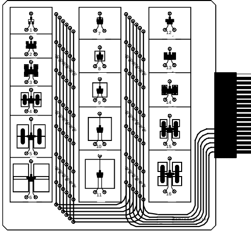
Figure 2. Top Side of the 4.5"x5" SuperSOT™-3 Thermal Board. Complete scale drawings are shown in section 5.
