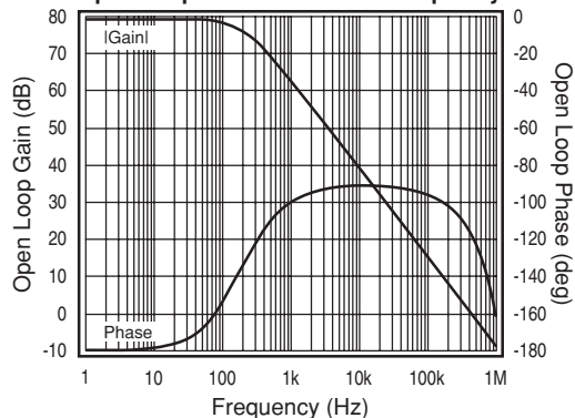
Open Loop Gain &amp; Phase vs. Frequency
