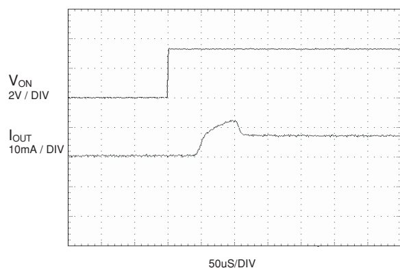
Figure 15. Turn-On Response
