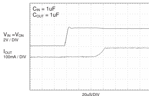
Figure 20. Current-Limit Response
