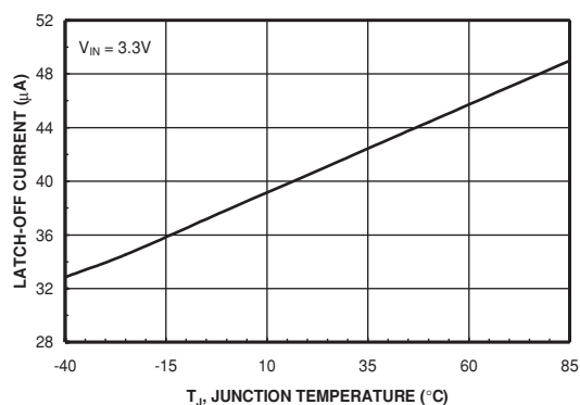
Figure 7. Latch-Off Current vs. Temperature
