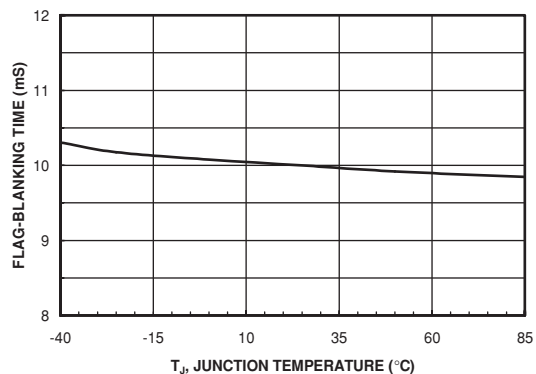
Figure 17. Blank Time vs. Temperature
