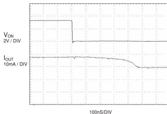
Figure 16. Turn-Off Response
