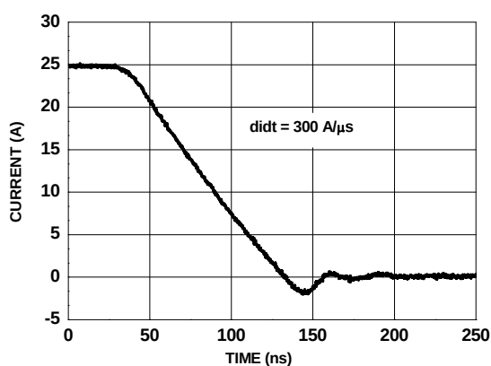
Figure 27. FDMS3664S SyncFET body diode reverse recovery characteristic
