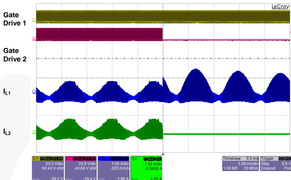
Figure 29. Phase-Shedding Operation
