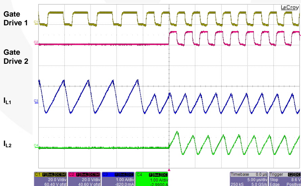
Figure 31. Phase-Adding Operation
