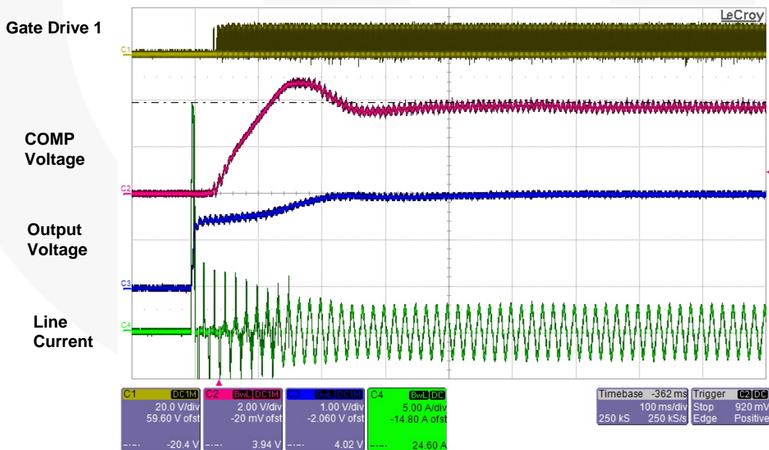
Figure 16. Full-Load Startup at 230V AC
