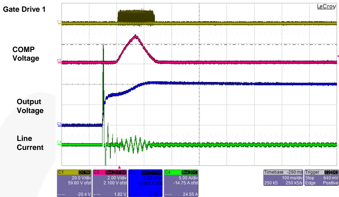
Figure 15. No-Load Startup at 230V AC
