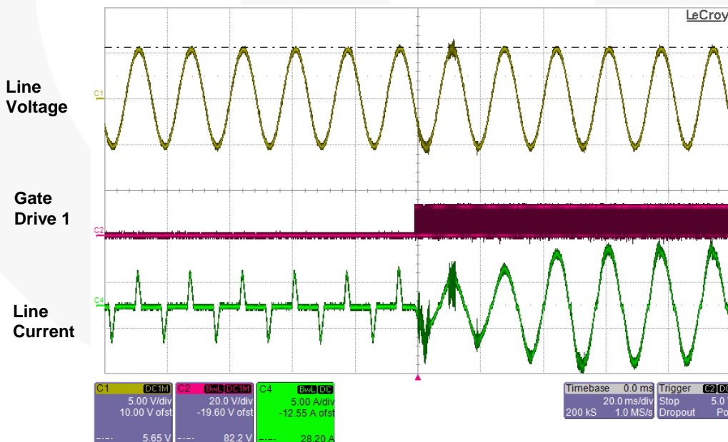
Figure 25. Startup Slowly Increasing the Line Voltage
