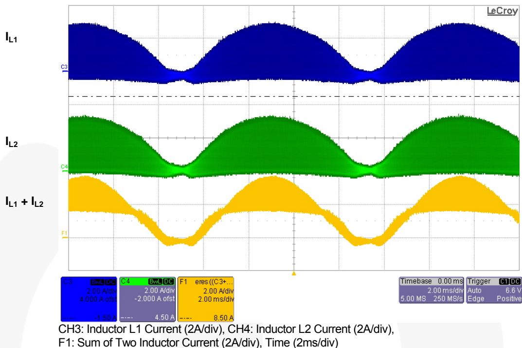
Figure 19. Inductor Current Waveforms at Full-Load and 230V AC
