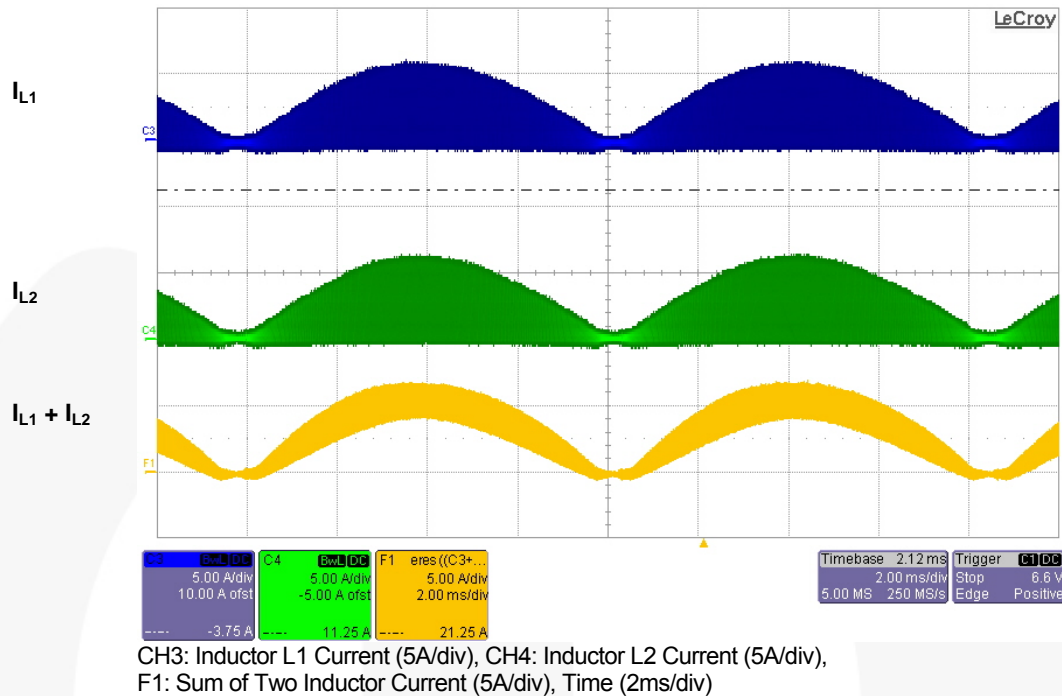
Figure 17. Inductor Current Waveforms at Full-Load and 115V AC
