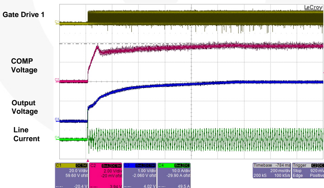
Figure 13. No-Load Startup at 115V AC
