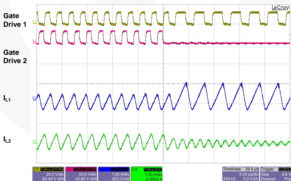
Figure 29. Phase-Shedding Operation
