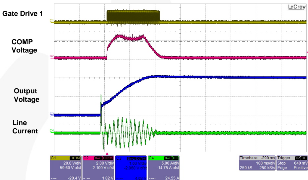
Figure 13. No-Load Startup at 115V AC
