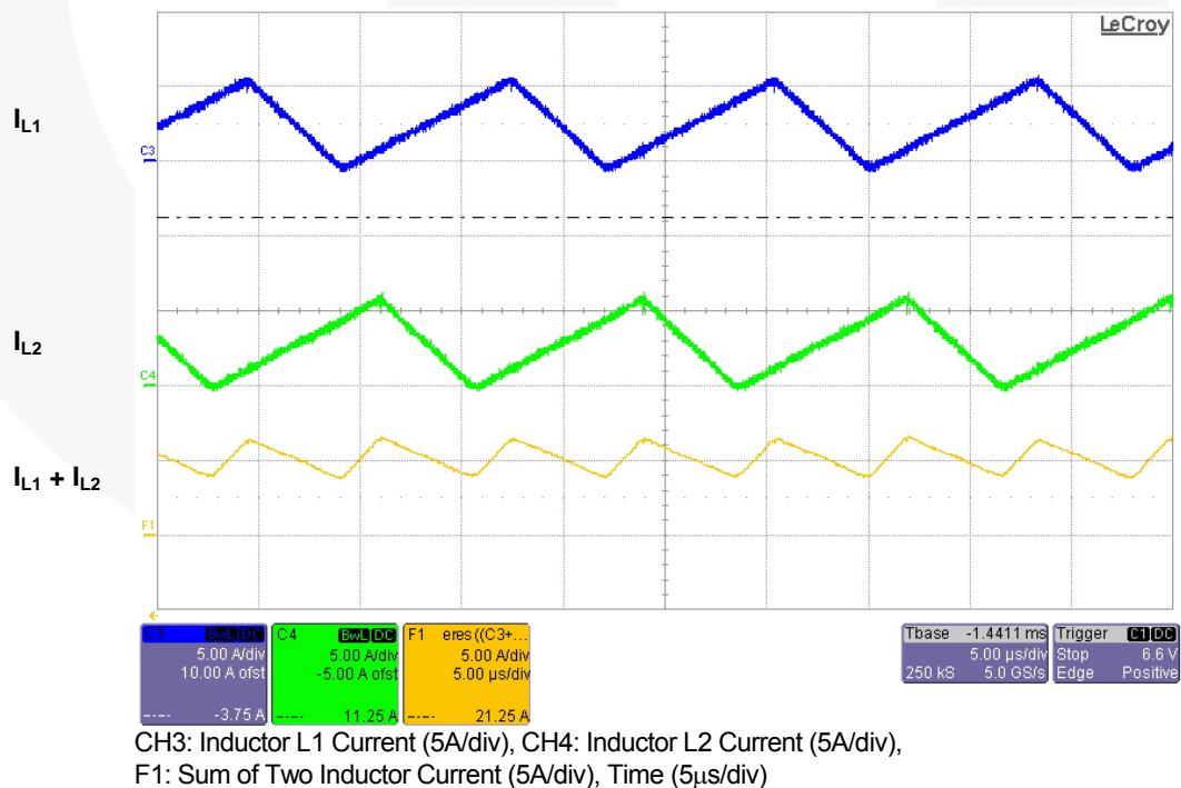
Figure 18. Zoom of Inductor Current Waveforms of Figure 17 at Peak of Line Voltage
