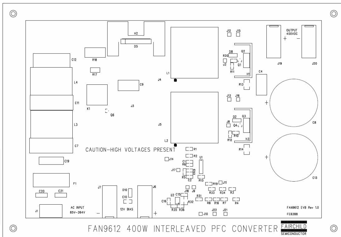
Figure 11. Top Silkscreen
