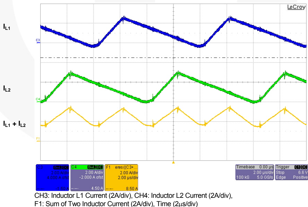
Figure 20. Zoom of Inductor Current Waveforms of Figure 19 at Peak of Line Voltage
