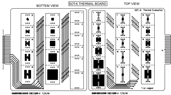
Figure 2. Both Sides of the 4.5"x5" SuperSOT™-6 Thermal Board. Complete scale drawings are shown in Section 5.
