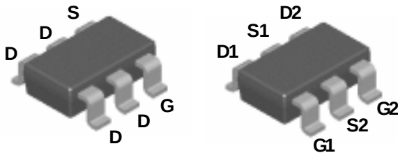
Figure 1. SuperSOT™-6 Power MOSFET achieves junction-to-case thermal resistance R_{\theta JC} of 30°C/W for single device and 60°C/W for dual devices.
