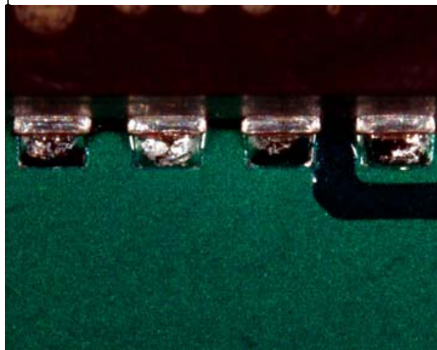
Figure 2: Solder wetted to lead-frame copper exposed by singulation on lead ends.
