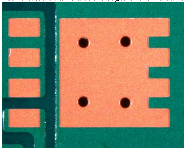
Figure 3: PWB pad showing OSP pad finish and vias.
