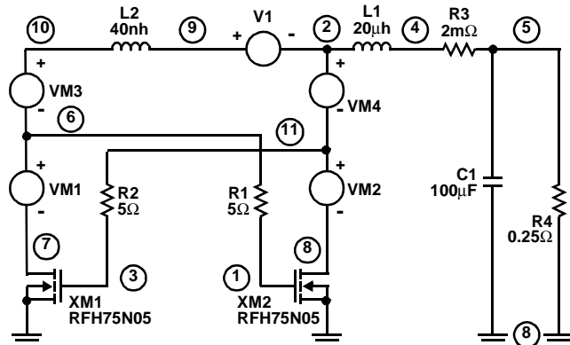
FIGURE 2. SYNCHRONOUS RECTIFIER CIRCUIT
