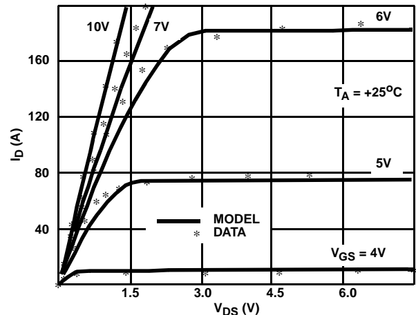
FIGURE 9. OUTPUT CURVES
