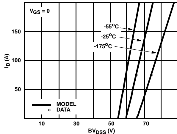
FIGURE 13. BREAKDOWN VOLTAGE, HIGH CURRENT BV_{DS} Excellent agreement exists.
