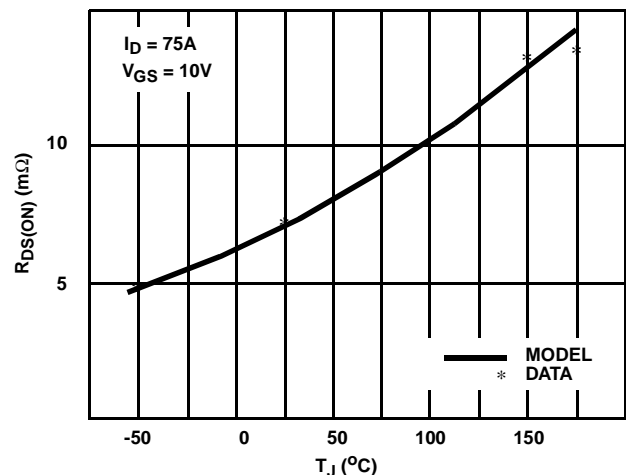
FIGURE 14. ON RESISTANCE vs TEMPERATURE Excellent agreement exists.
