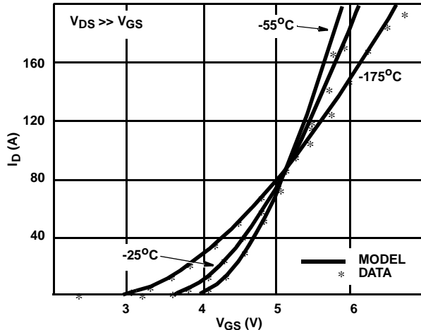
FIGURE 10. TRANSFER CURVES
