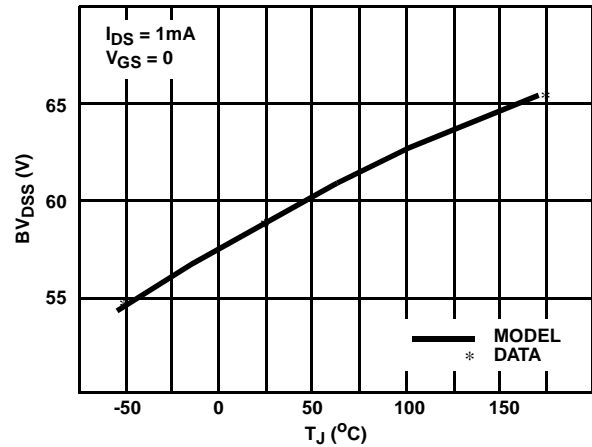
FIGURE 12. BREAKDOWN VOLTAGE, LOW CURRENT BV_{DS} Excellent agreement exists.
