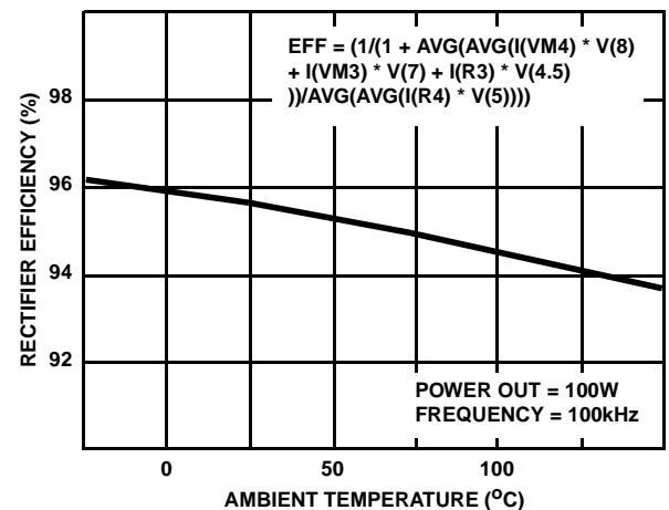
FIGURE 4. RECTIFIER EFFICIENCY
