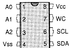
Plastic Dual-in-line "P" Package
