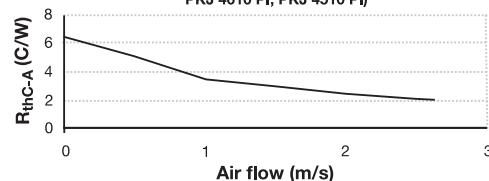
Case to Ambient Thermal Resistance for 2.5V and 3.3V (PKJ 4719 PI, PKJ 4519 PI, PKJ 4319 PI, PKJ 4910 PI, PKJ 4610 PI, PKJ 4510 PI)
