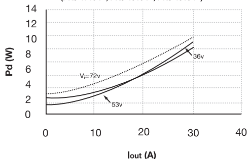
Power Loss vs. Output Current for 2.5V (PKJ 4719 PI, PKJ 4519 PI, PKJ 4319 PI)
