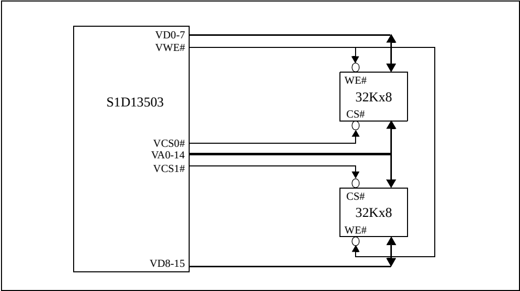
Figure 48: 16-Bit Mode - 64K bytes SRAM
