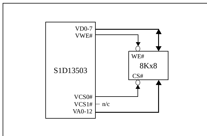
Figure 42: 8-Bit Mode - 8K bytes SRAM
