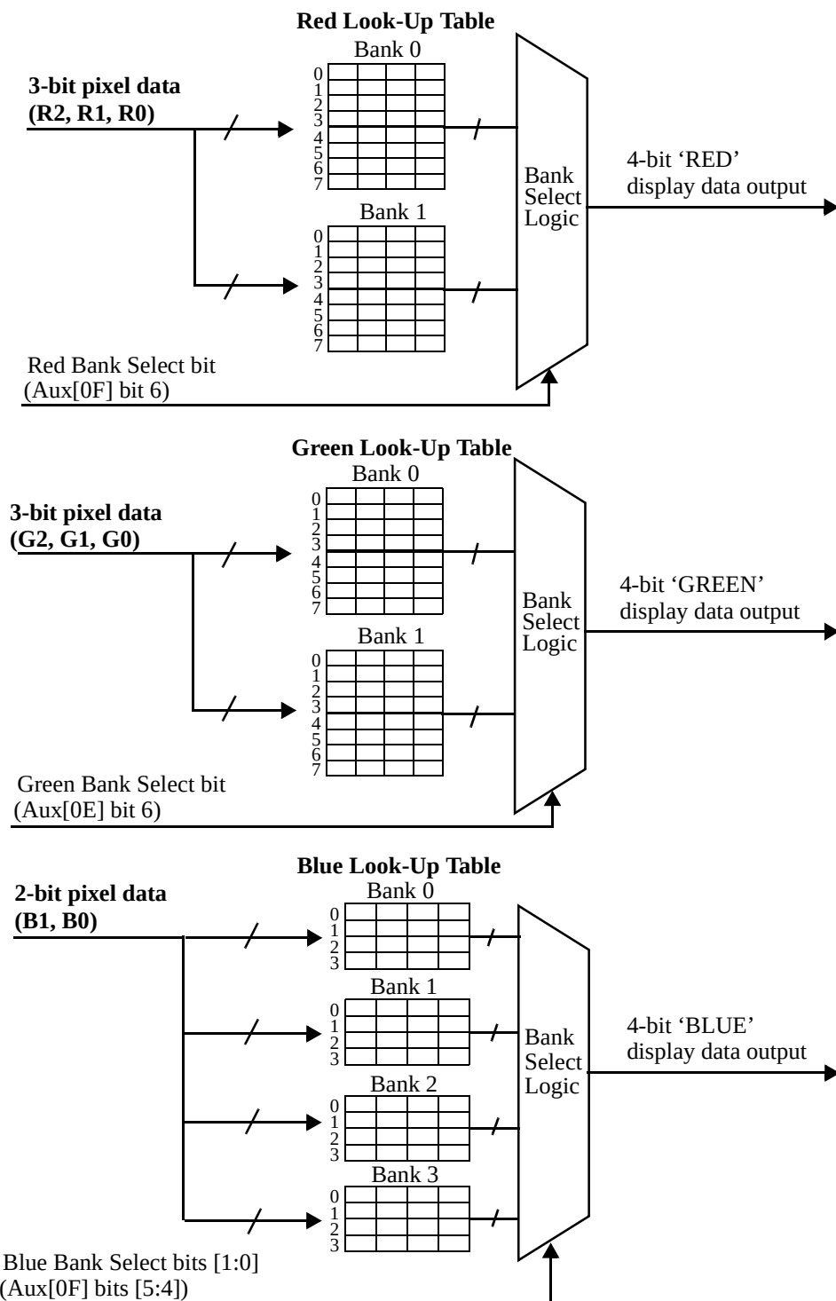
Figure 9: 256-Level Color Mode Look-Up Table Architecture
