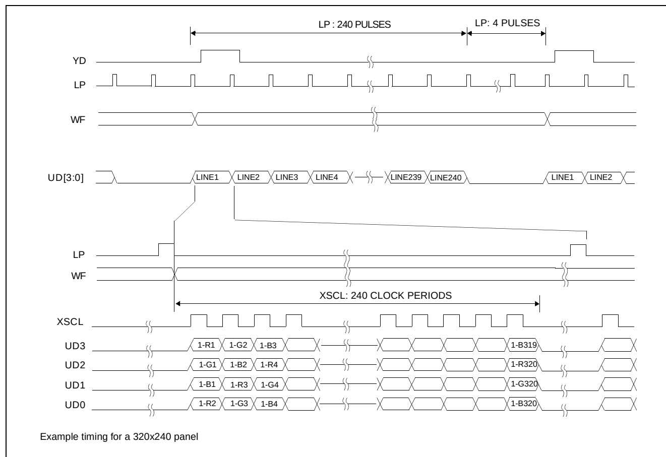
Figure 30: 4-Bit Single Color Panel Timing
