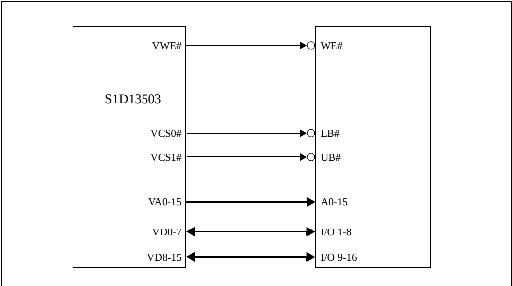
Figure 49: 16-Bit Mode - 128K bytes SRAM
