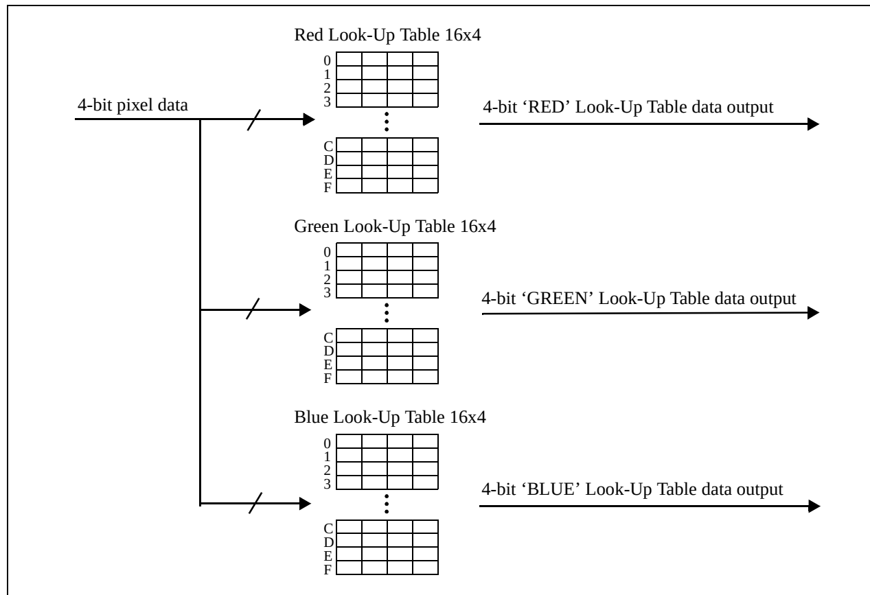
Figure 40: 16-Level Color Mode Look-Up Table Architecture
