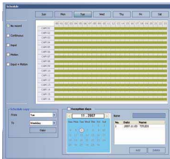
Figure 6.34 The Exception day setting window
