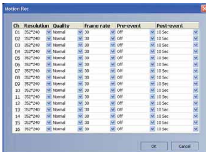
Figure 6.30 The Motion recording setting window
