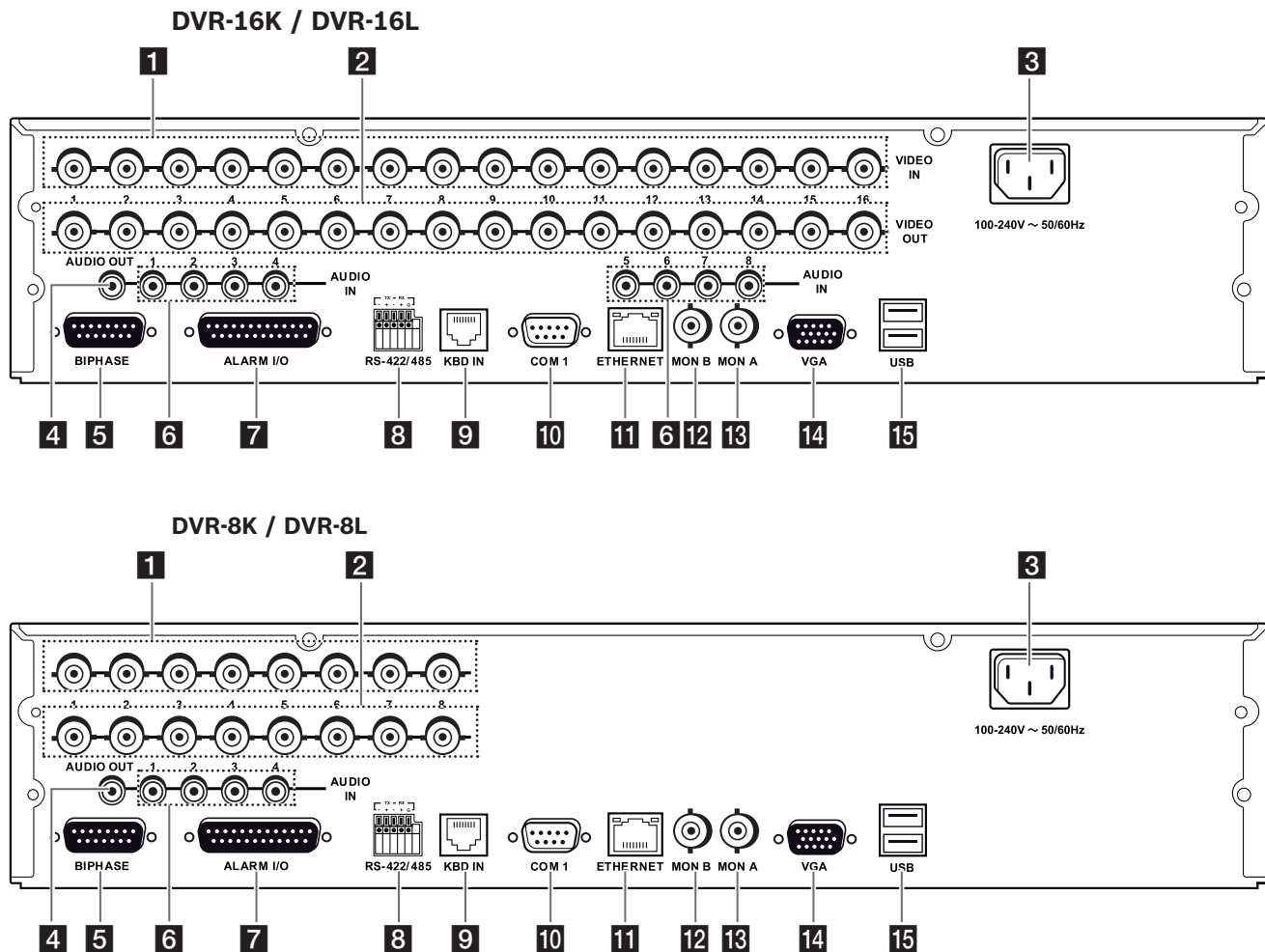
Figure 2.3 Back panel
