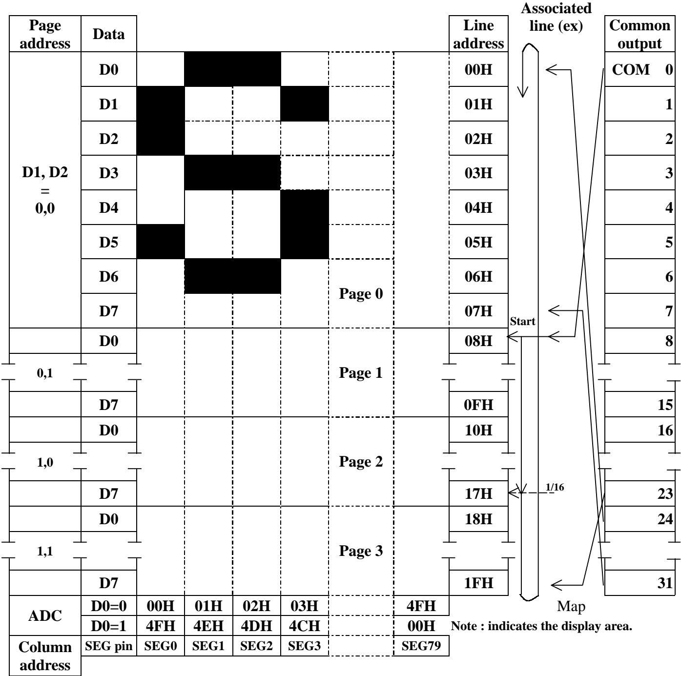
Display Data RAM Addressing
