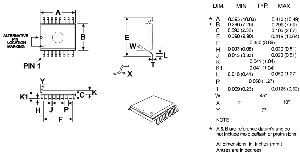
Figure 7 16-pin SOIC (D4) Mechanical Outline: Order as part no. CMX654D4
