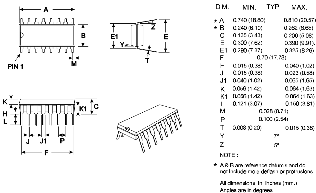
Figure 8 16-pin DIL (P3) Mechanical Outline: Order as part no. CMX654P3
