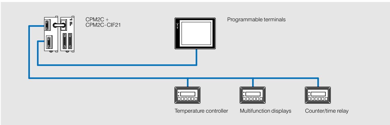
Device connection overview for CPM2C with CIF21
