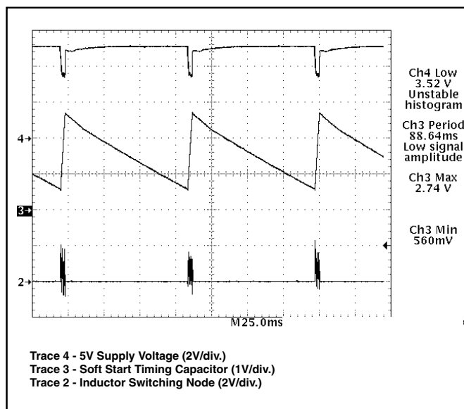
Figure 10: CS5157 demonstration board hiccup mode short circuit protection. Gate pulses are delivered while the soft start capacitor charges, and cease during discharge.
