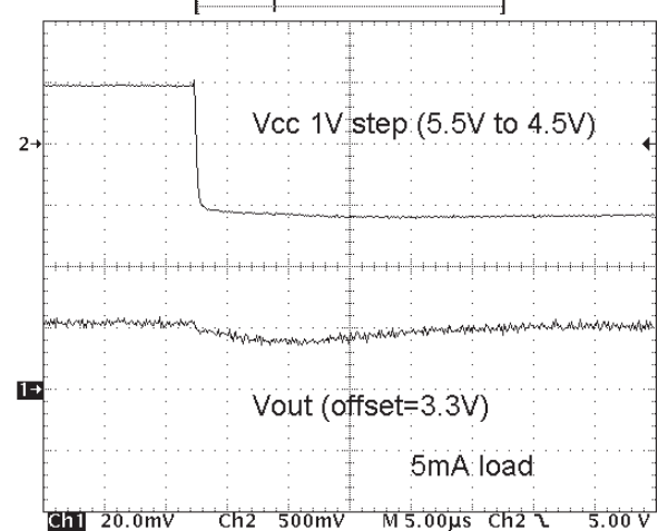
Fig 2.16 V_{CC} Load Step Response Falling
