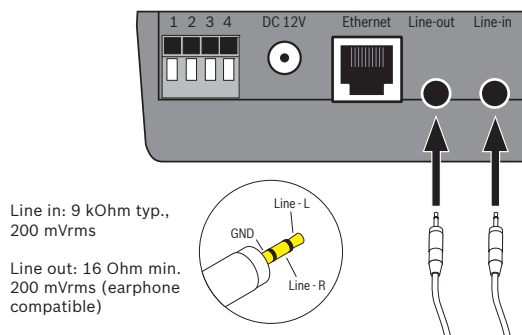
Figure 3.5 Audio connectors
