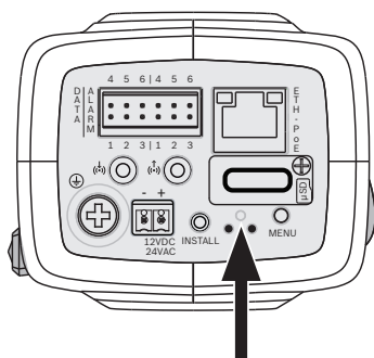
Figure 7.1 Reset button
