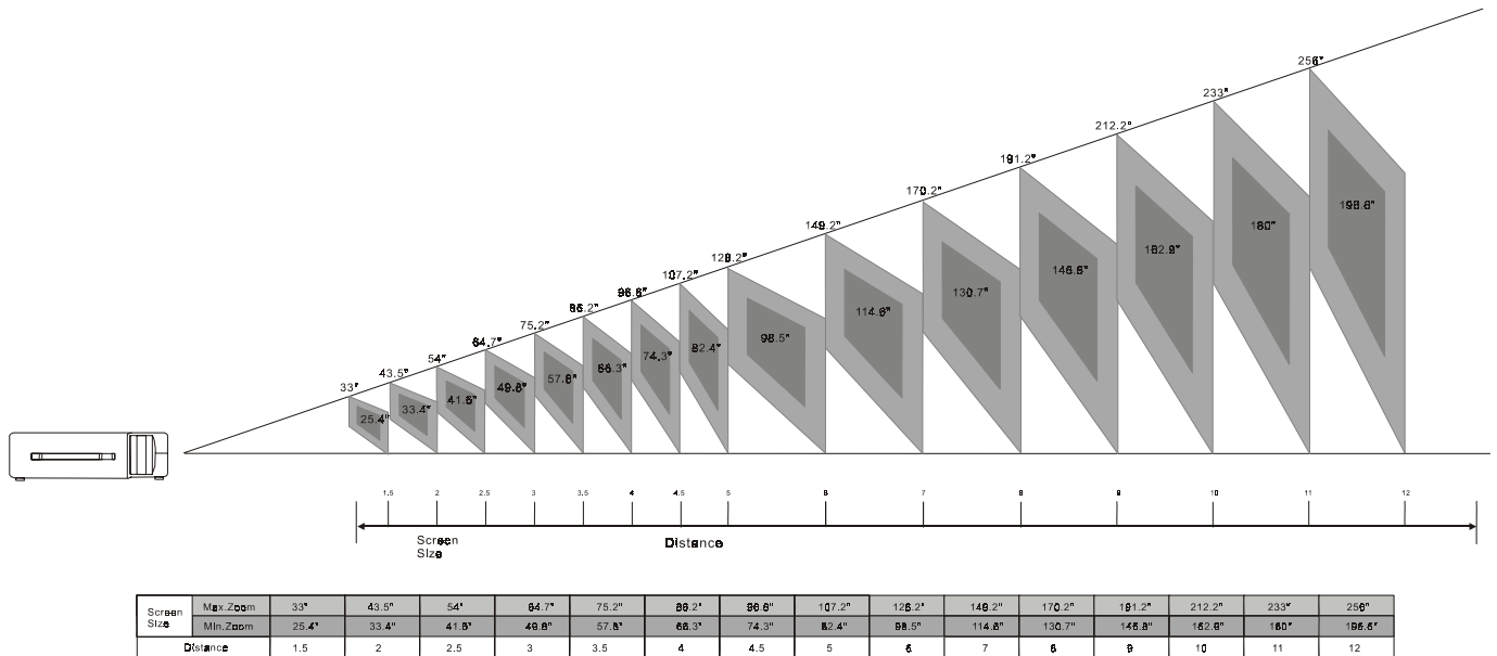
Figure 4 Positioning of 7763P/65PE
