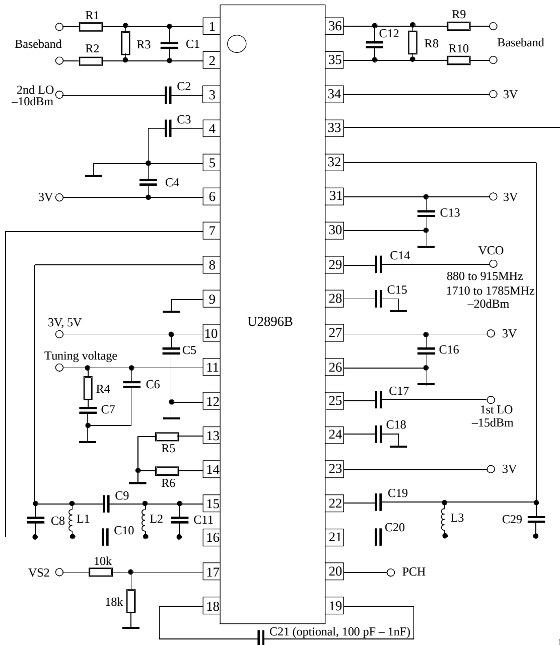
Figure 15. Application circuit
