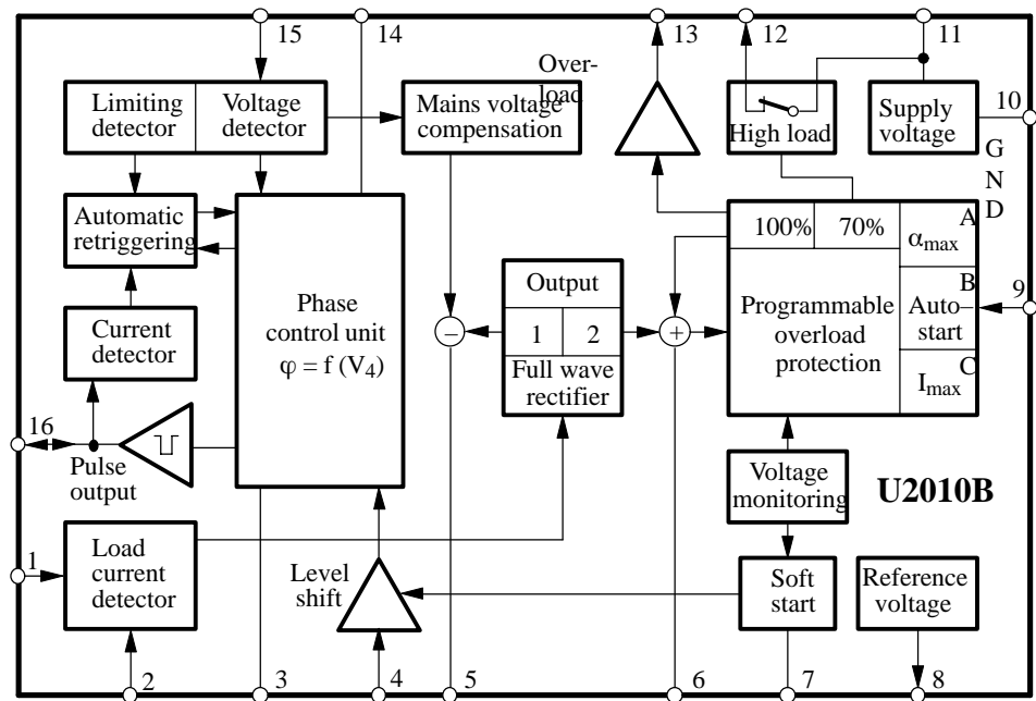
Figure 1. Block diagram
