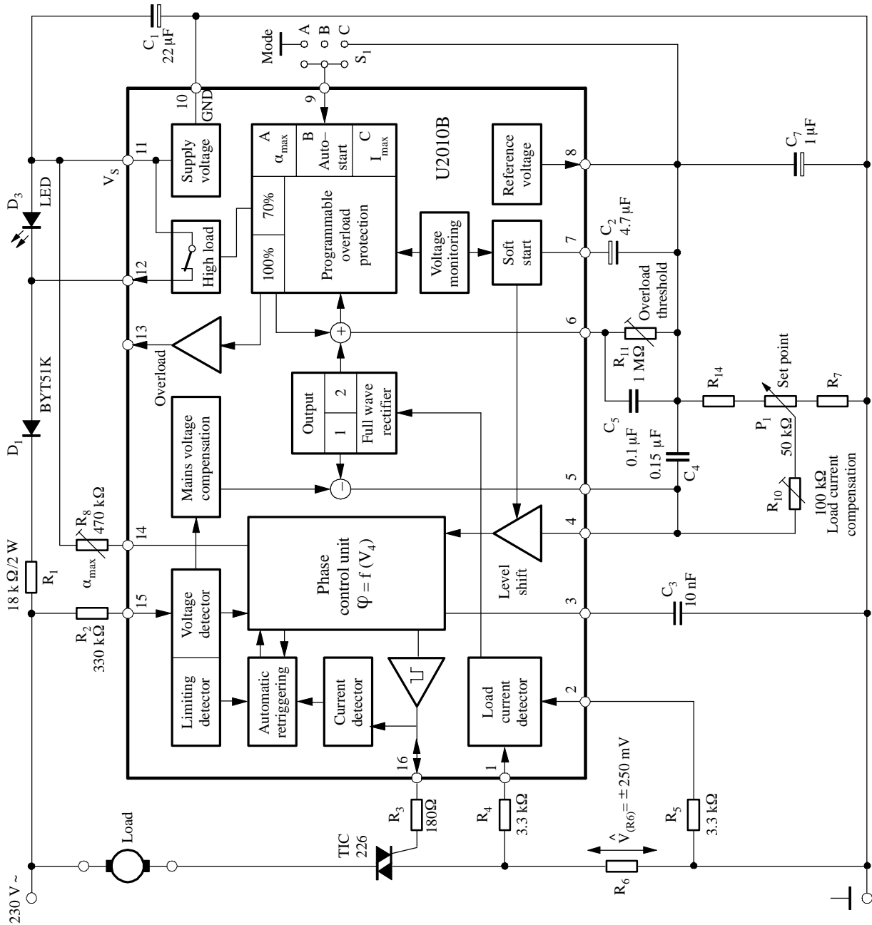
Figure 2. Block diagram with external circuit
