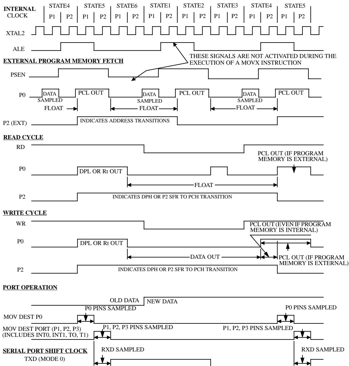
Figure 33. Clock Waveforms
