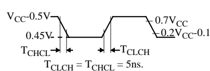
Figure 24. Clock Signal Waveform for I_{CC} Tests in Active and Idle Modes
